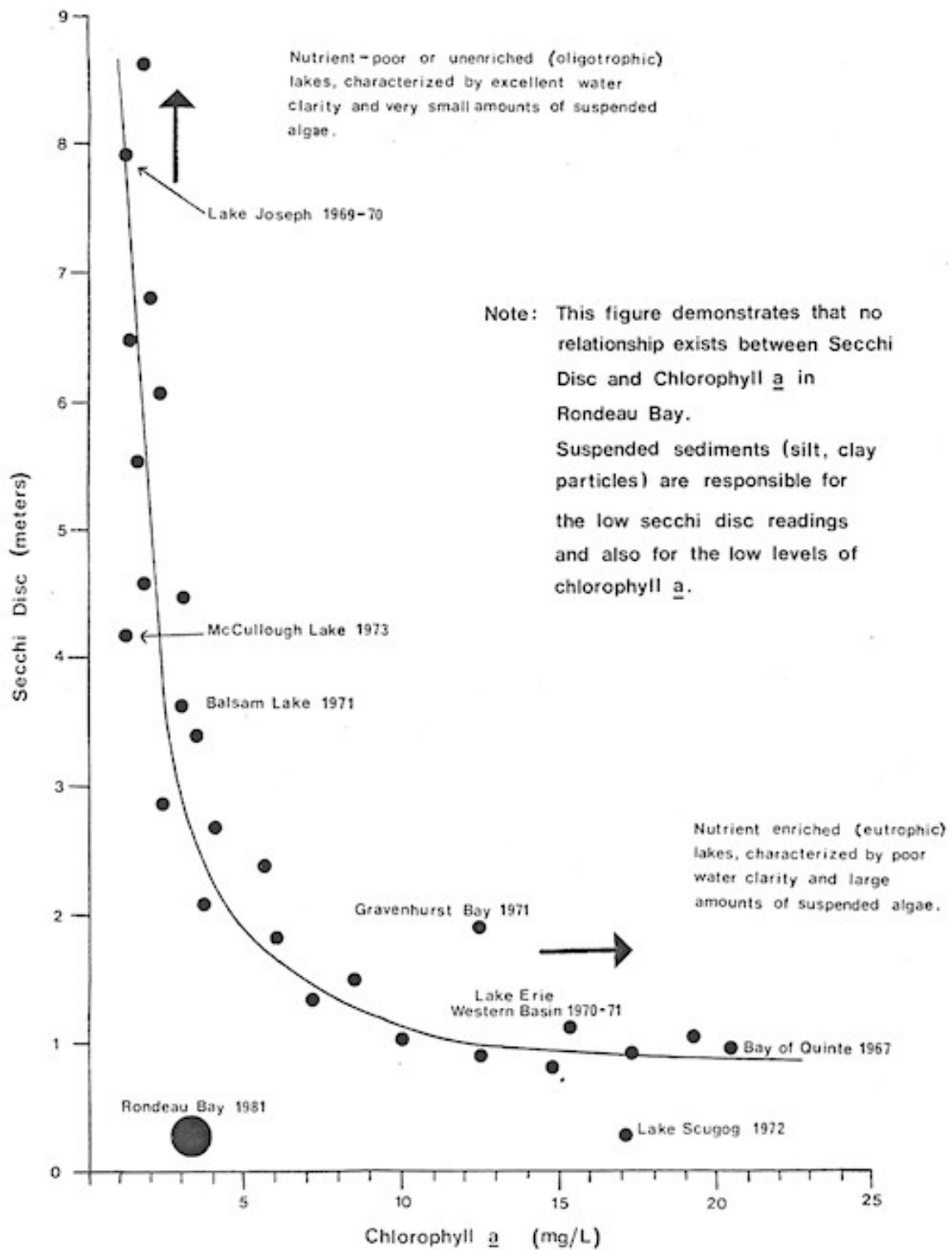
Figure 3. Relationship between Secchi Disc and Chlorophyll a for a number of lakes in Ontario.
