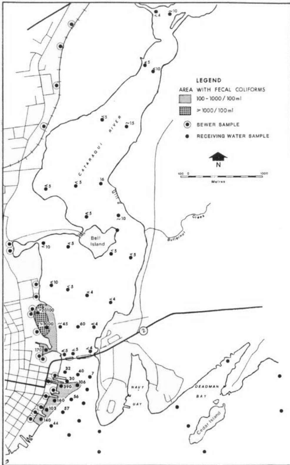
FIGURE10: Kingston Subgrid 1 Fecal Coliform Levels (org./100ml) August 8, 1985.
