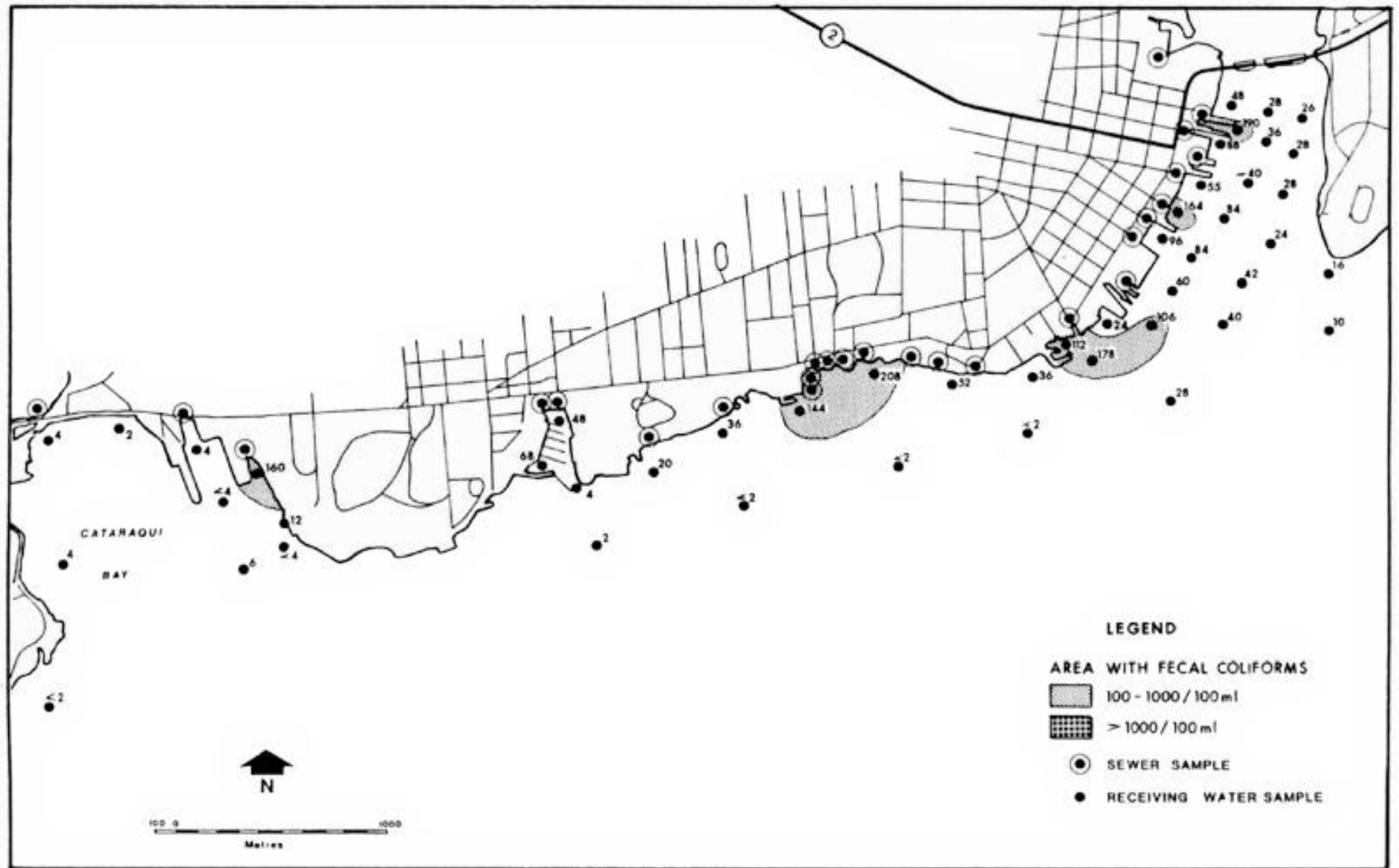
FIGURE12: Kingston Subgrid 2 Fecal Coliform Levels (org/100ml) August 14, 1985.
