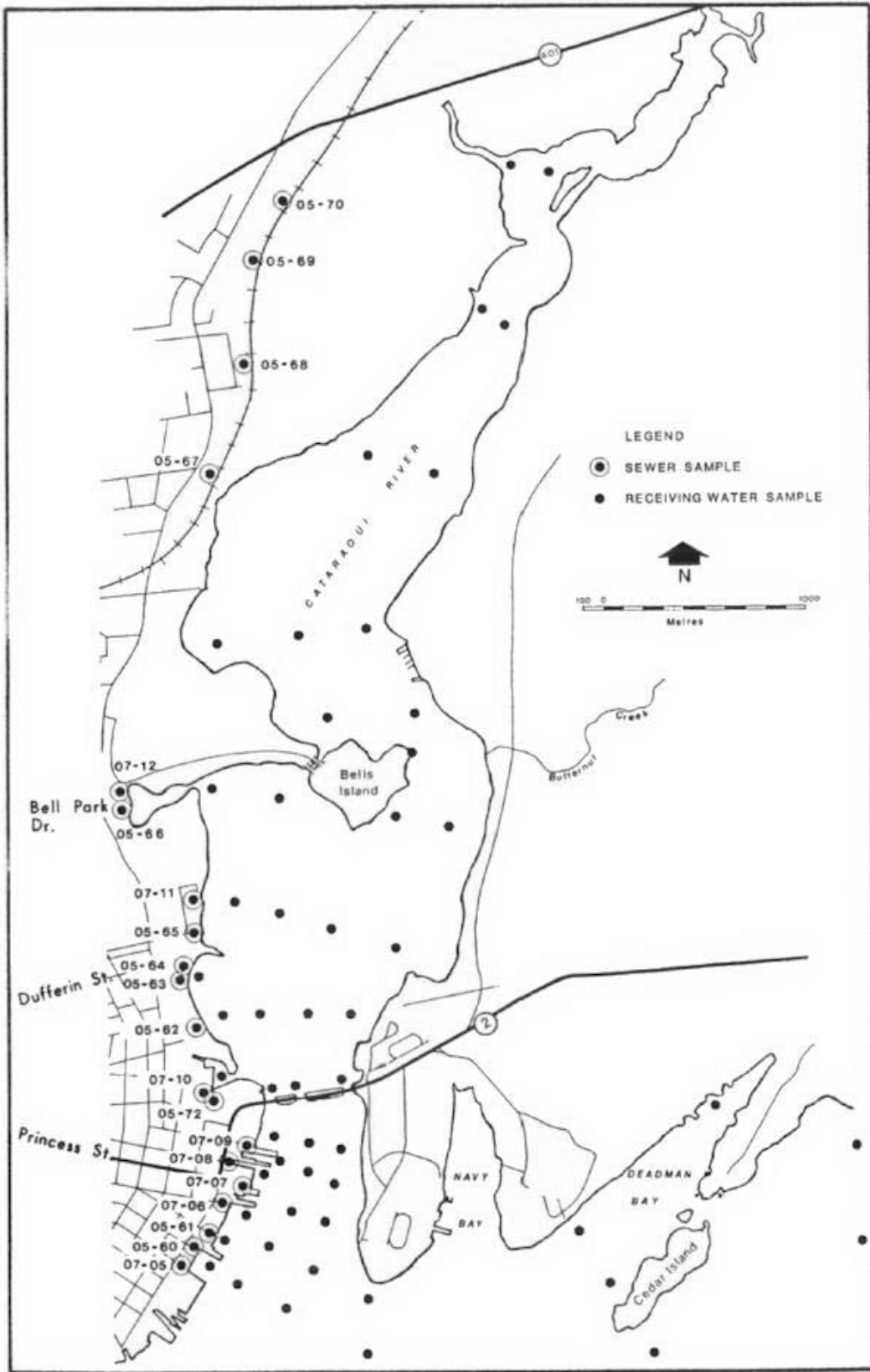
FIGURE 2 : 1985 Kingston Harbour Bacteriological Survey: Subgrid 1- Sampling Locations.
