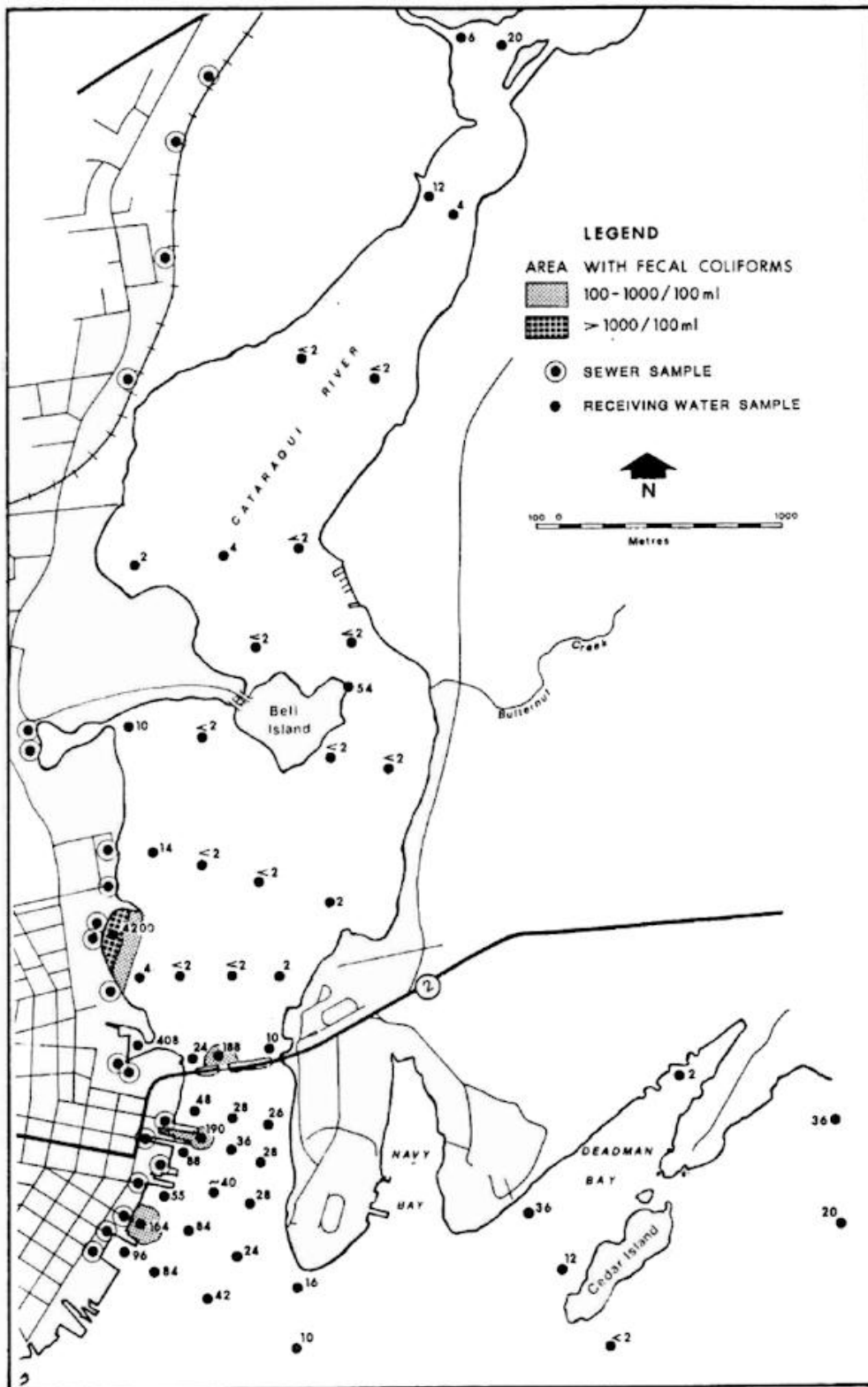
FIGURE 11: Kingston Subgrid 1 Fecal Coliform Levels (Org/100ml) August 14, 1985.
