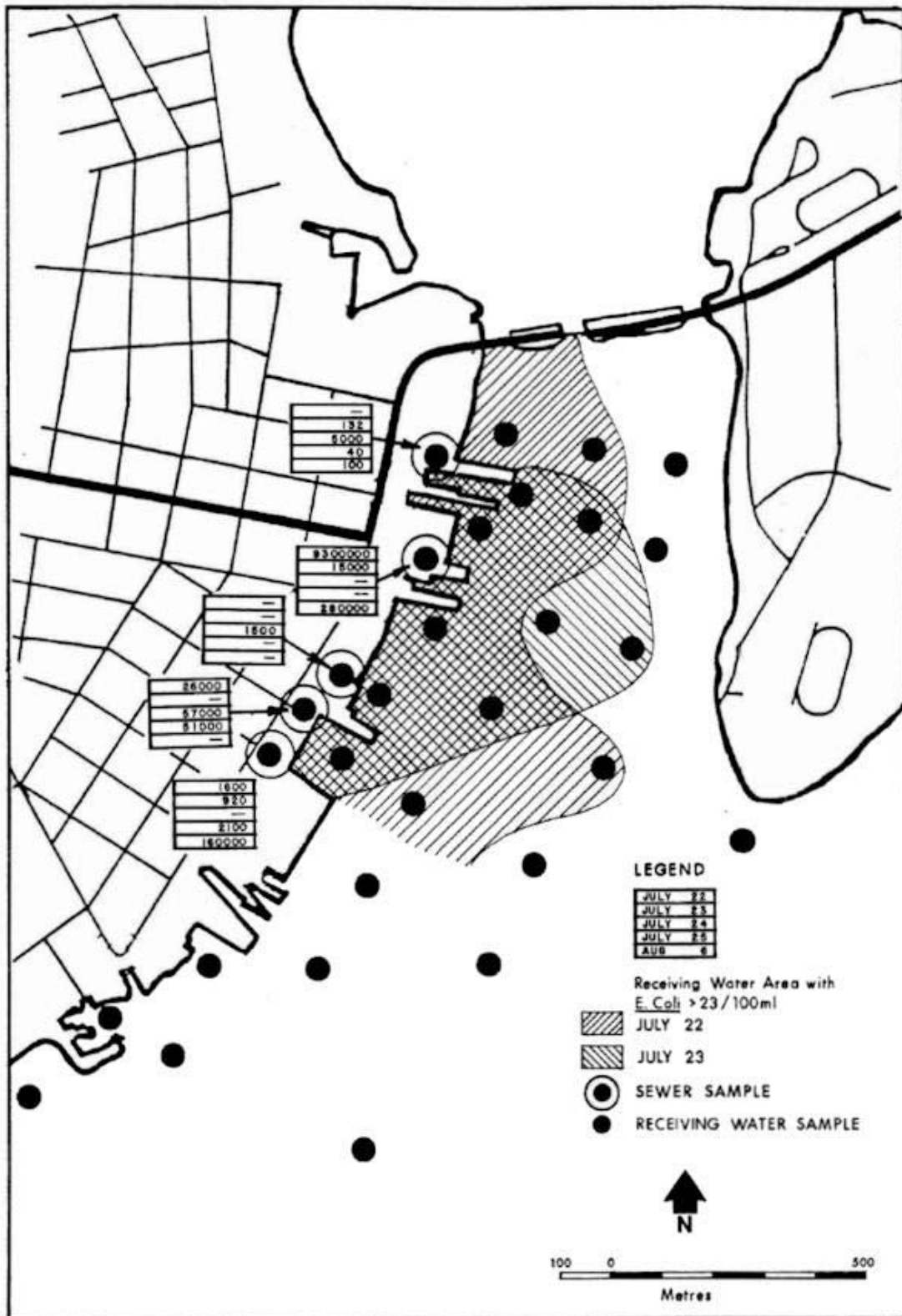
FIGURE 7: E. coli Counts (#/100ml Observed During Dry Weather Downtown Kingston Waterfront, 1986.
