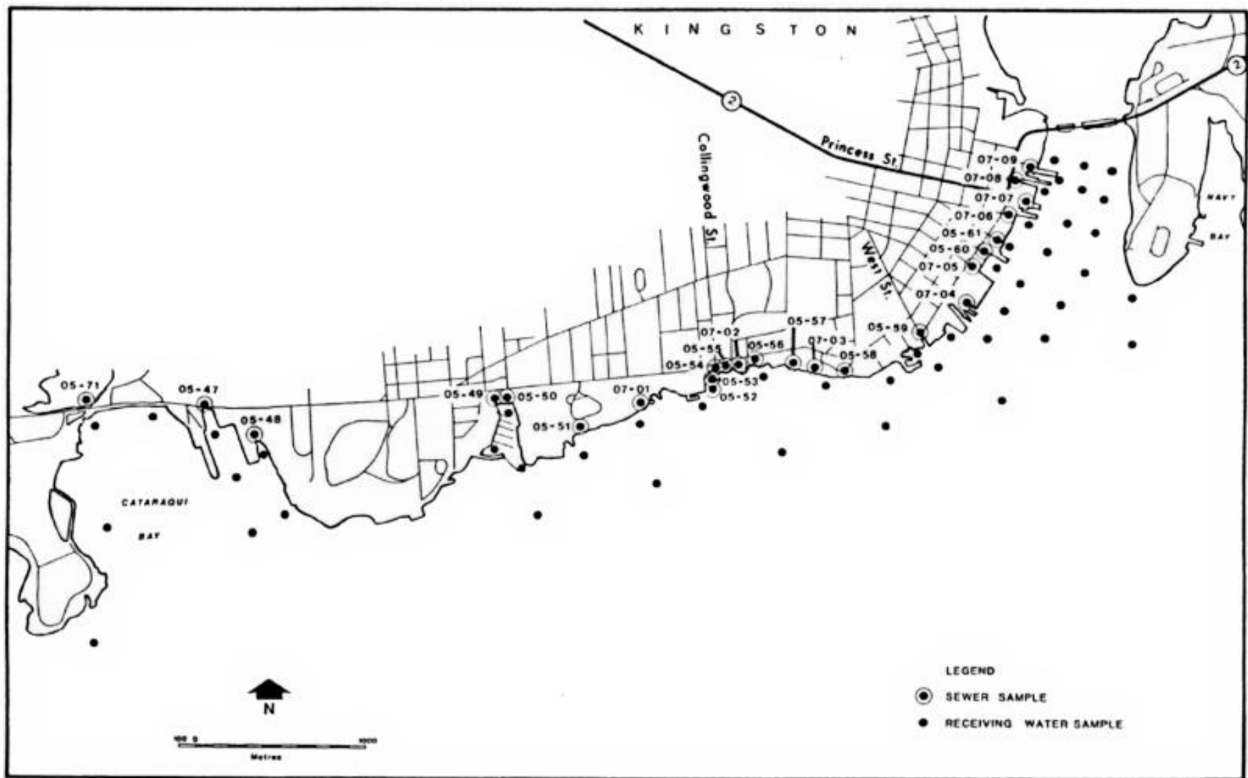
FIGURE 3 : 1985 Kingston Harbour Bacteriological Survey: Subgrid 2- Sampling Locations.
