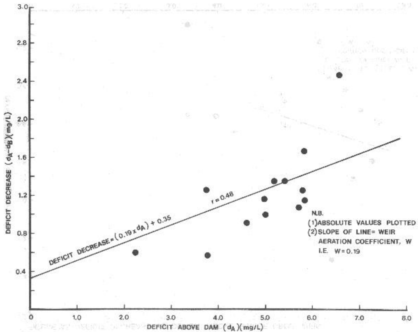
FIGURE A4: DEFICIT DECREASE VS DEFICIT ABOVE 5-STEP WEIR
