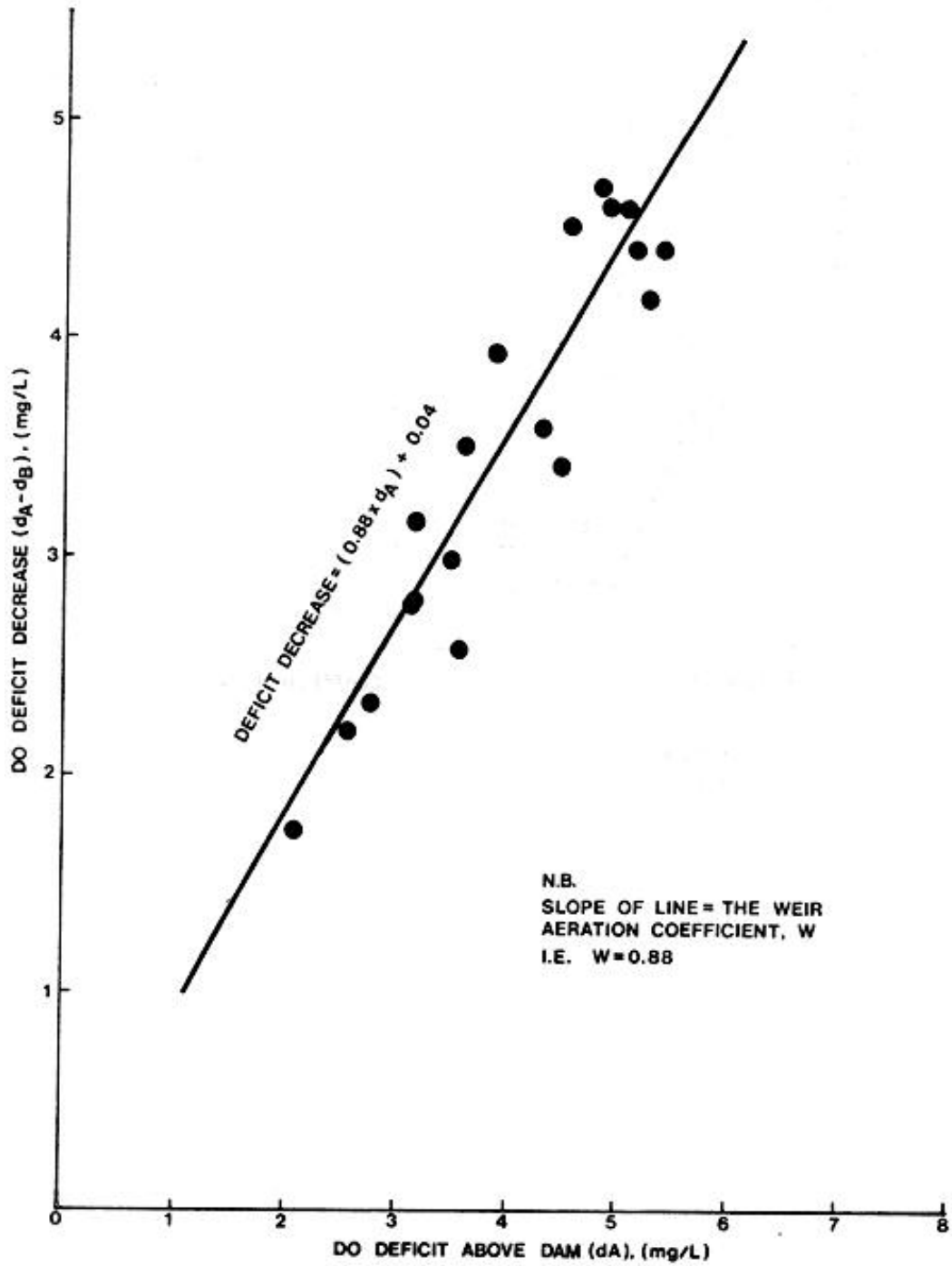
FIGURE A1: DO DEFICIT DECREASE VS DEFICIT ABOVE JOHN ST. WEIR (Strn. 6)
