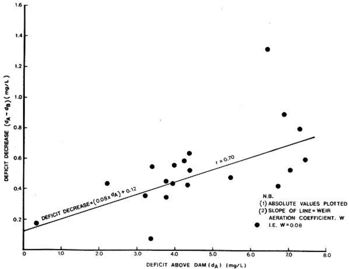
FIGURE A5: DEFICIT DECREASE VS DEFICIT ABOVE SINGLE DROP WEIR
