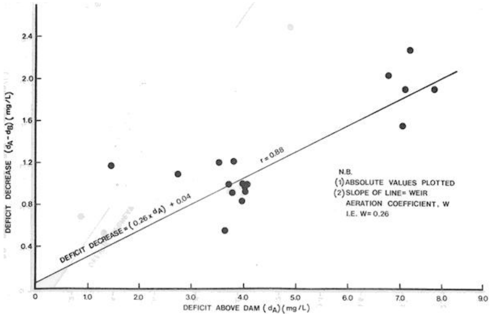
FIGURE A3: DEFICIT DECREASE VS DEFICIT ABOVE 3-STEP WEIR
