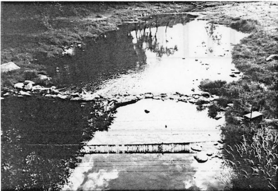
FIGURE 3: BROAD-CRESTED ROCK DAM AT STATION 10
