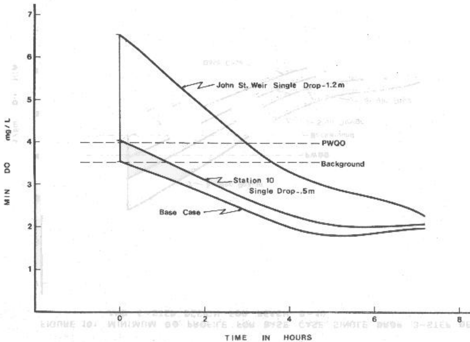
FIGURE 9: MINIMUM DO PROFILE FOR BASE CASE AND 2 SINGLE DROP WEIRS OF DIFFERENT HEIGHTS FOR REACH 9-10
