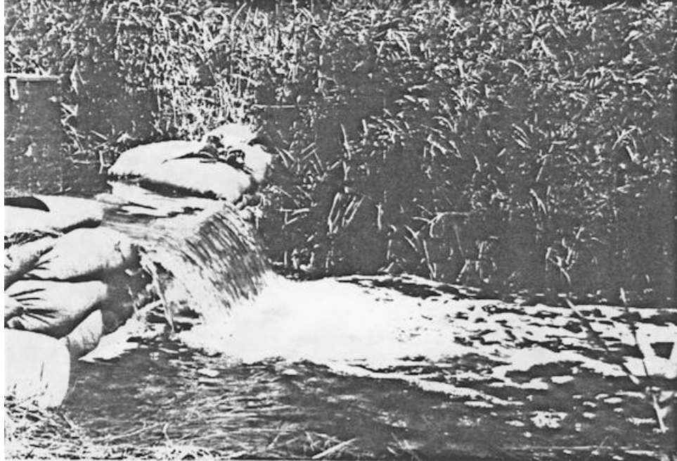
FIGURE 7: SINGLE DROP DESIGN WEIR
