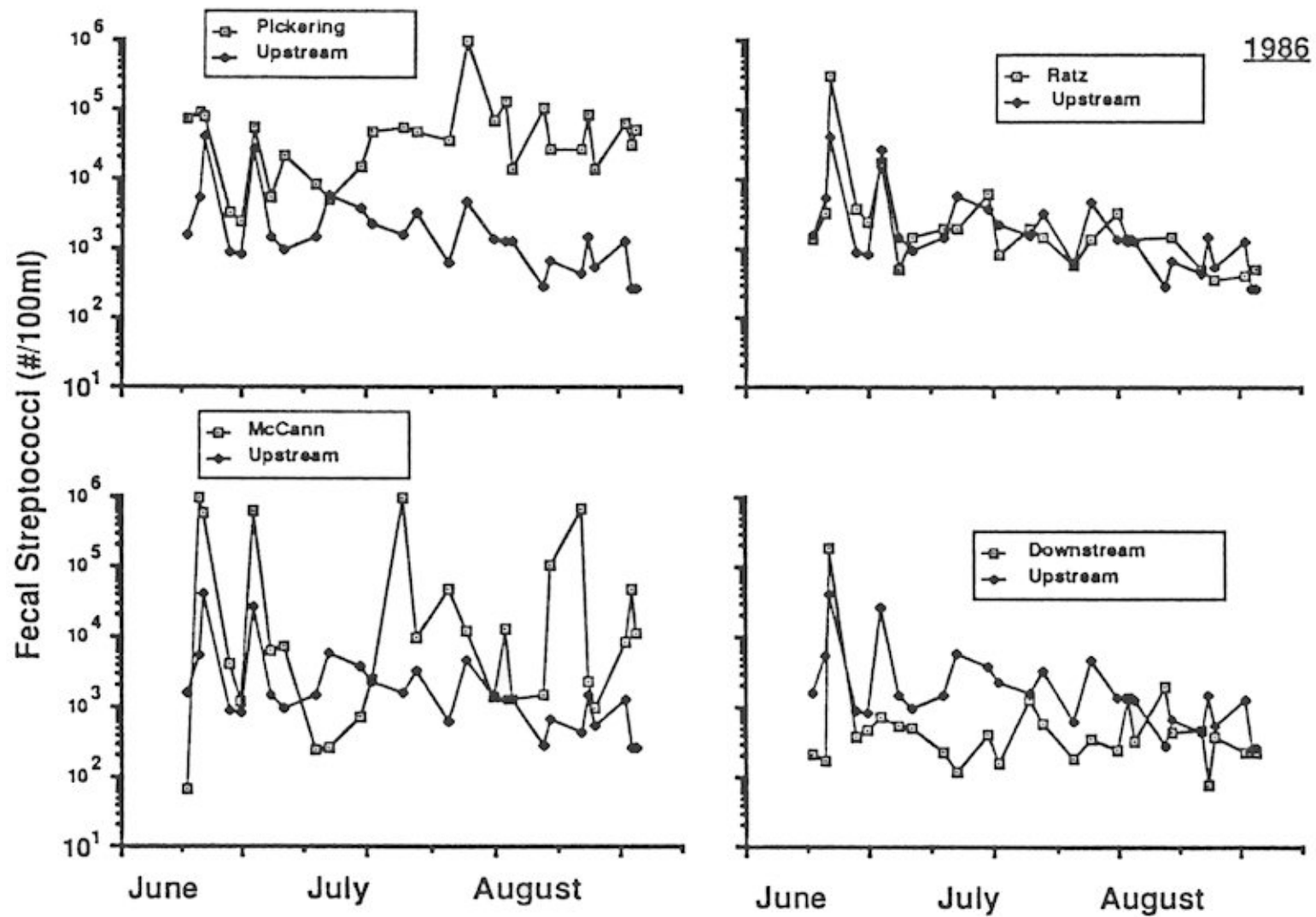
Figure 4: Concentration of fecal streptococci at five sampling sites along the Desjardine Drain from June through August, 1986. See Figure 1 for location of sampling sites.
