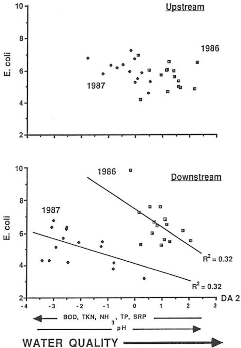
Figure 8: Relationships between concentration (numbers per 100 mL.) of E. coli (log axis) and water quality as represented by discriminant axis 2 (see Figure 6) at the Upstream and Downstream sites in 1986 and 1987. See Figure 1 for location of sites.
