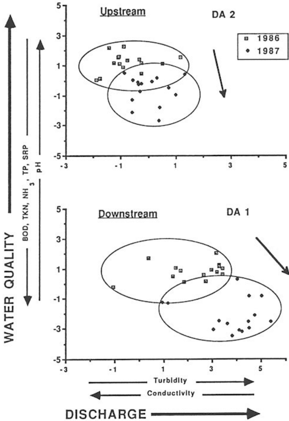
Figure 6: Plot of sampling sites in discriminant space in 1986 and 1987 as defined by water chemistry measurements. Each point represents a single sample.
