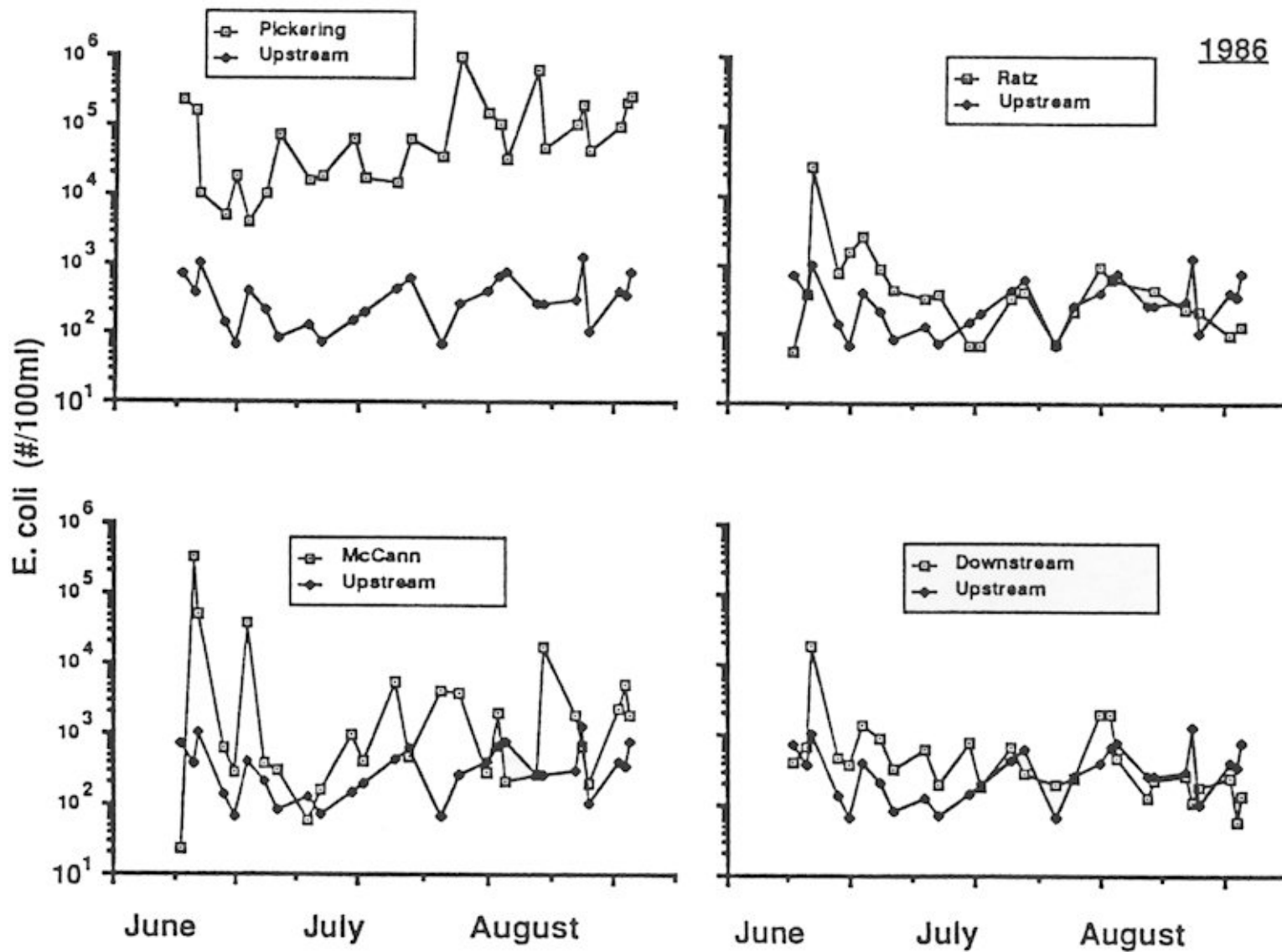
Figure 2: Concentration of Escherichia coli at five sampling sites along the Desjardine Drain from June through August, 1986. See Figure 1 for location of sampling sites.
