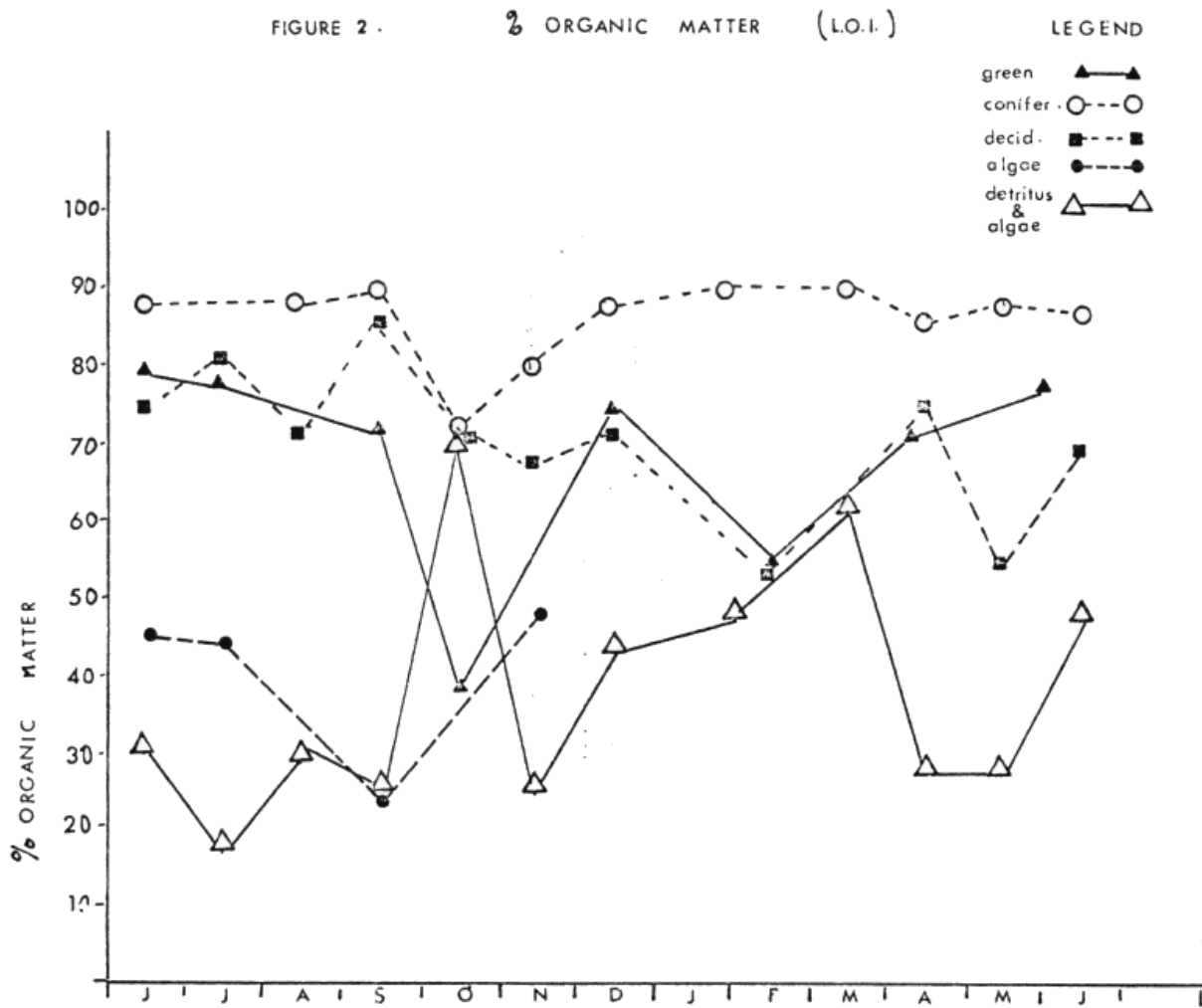
Figure 2. Annual fluctuations in percentage organic matter as determined by loss on ignition for station 2 monthly bulked samples. C.S.O.M. fractions and F.S.O.M. detritus-algae fraction values are graphed.
