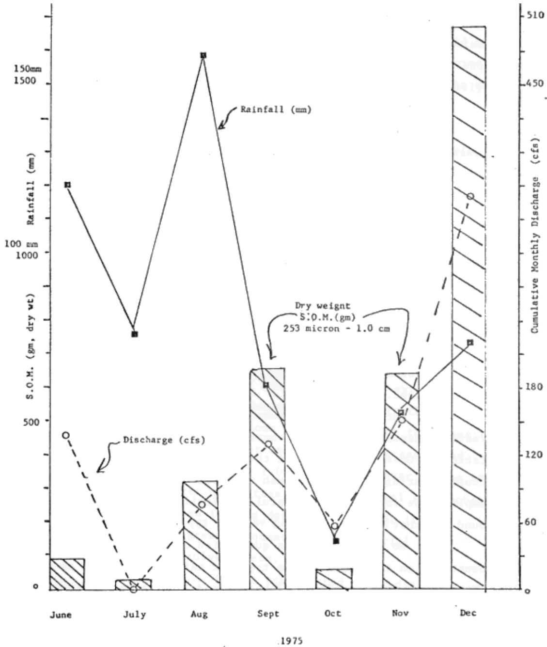
Figure 5. Relationship between rainfall, discharge and quantities of drifting S.O.M. (253 micron - 1.0 cm) on a monthly basis at Station 3 during 1975
