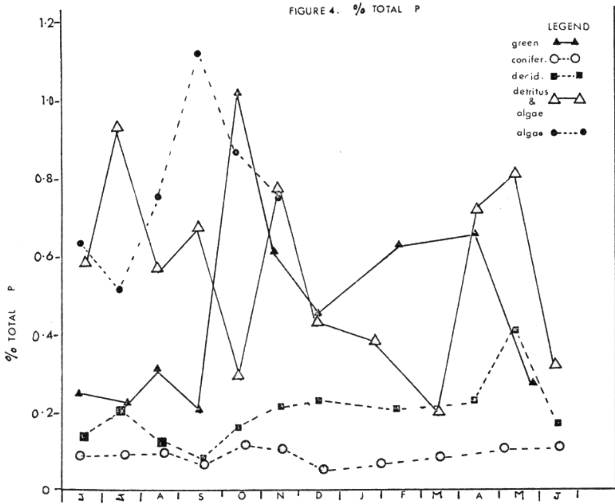
Figure 4. Annual fluctuations in percentage total phosphorus in organic matter of station 2 monthly bulked samples. C.S.O.M. fractions and F.S.O.M. detritus-algae fraction values are graphed.
