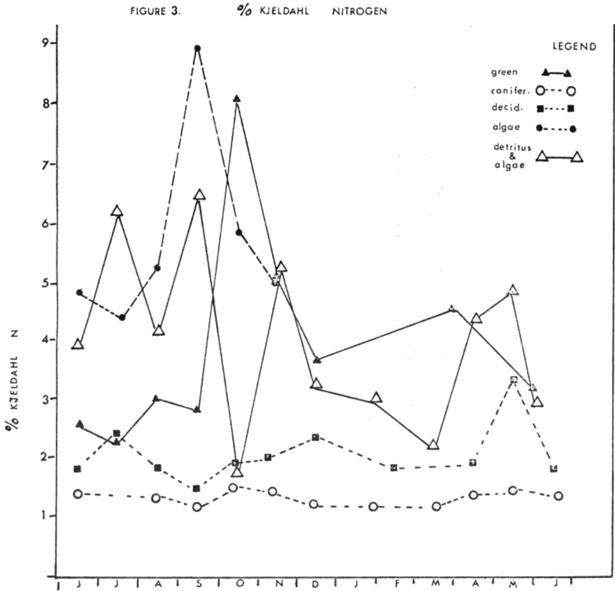
Figure 3. Annual fluctuations in percentage Kjeldahl nitrogen in organic matter of station 2 monthly bulked samples. C.S.O.M. fractions and F.S.O.M. detritus-algae fraction values are graphed.
