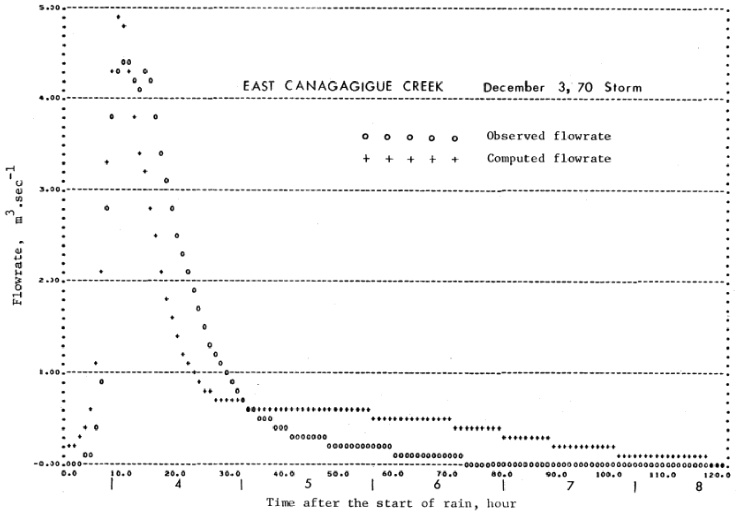
Fig. 18: Comparison of Observed and Simulated Flowrates Due to December 3, 1970 Storm on East Canagagigue Watershed.
