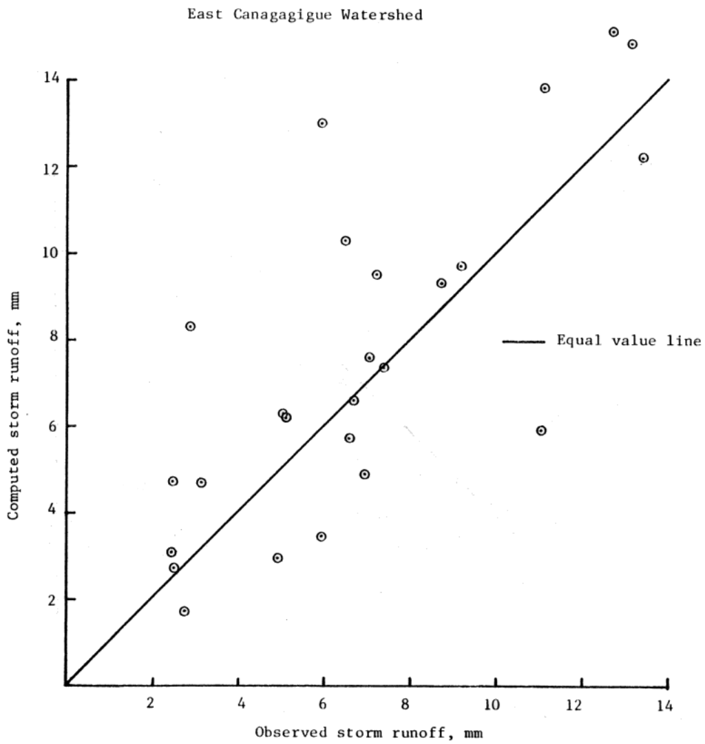
Fig. 24: Comparison of Observed and Computed Storm Runoff for Various Storms on East Canagagigue Watershed.
