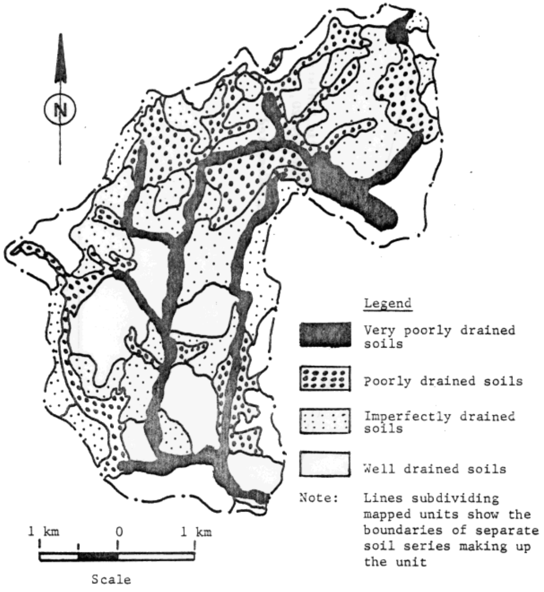
Fig. 7: Soil Map of Canagagigue (AG-4) Watershed.
