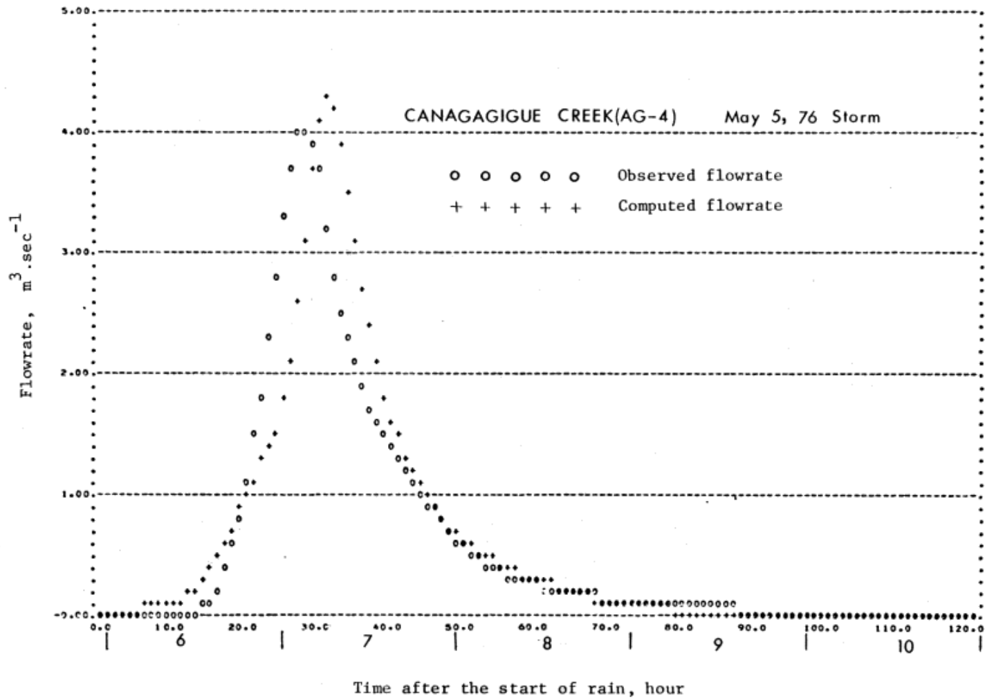
Fig. 17: Comparison of Observed and Simulated Flowrates due to May 5, 1976 Storm on Canagagigue (AG-4) Watershed.
