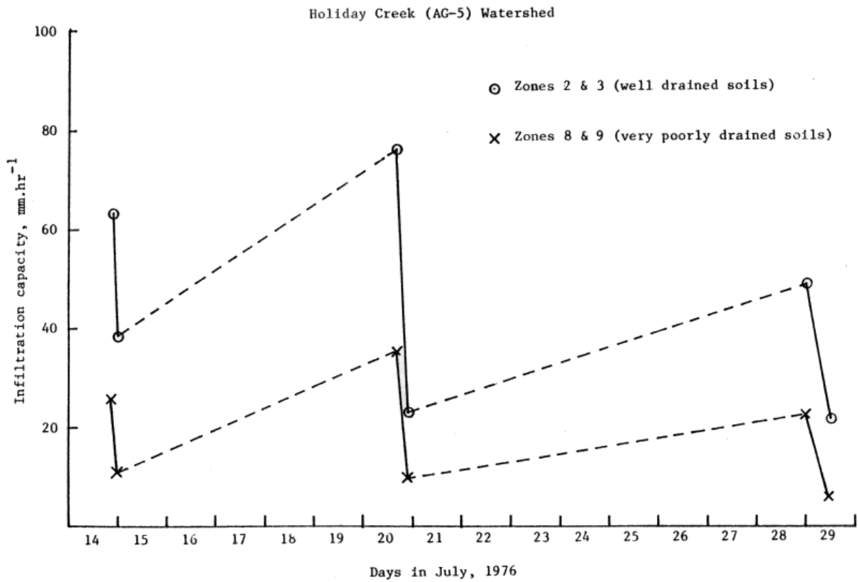
Fig. 41: Infiltration Capacity Rates During a Storm Sequence on Holiday Creek (AG-5) Watershed for July, 1976.
