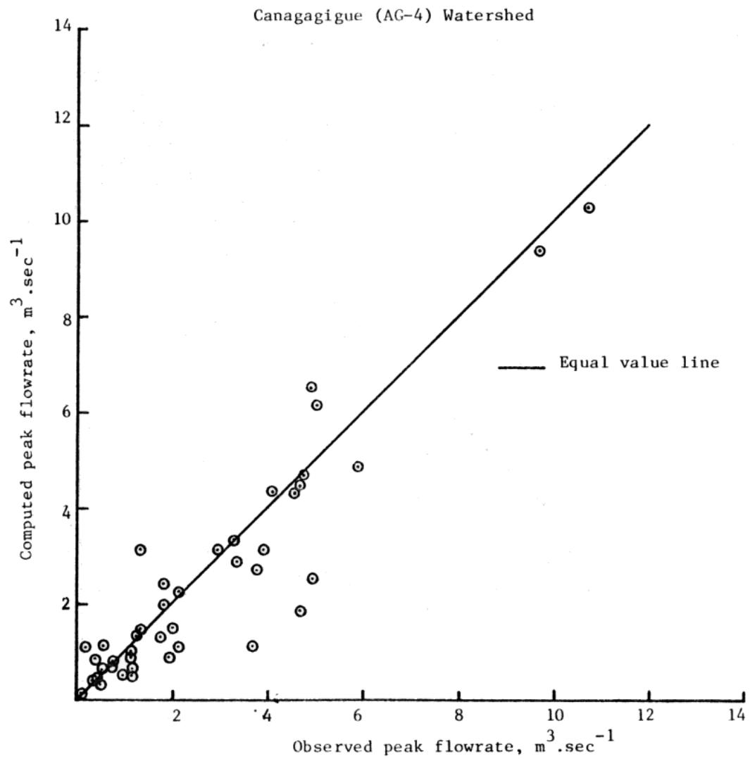
Fig. 20: Comparison of Observed and Computed Peak Flow-rates of Various Storms on Canagagigue (AG-4) Watershed.
