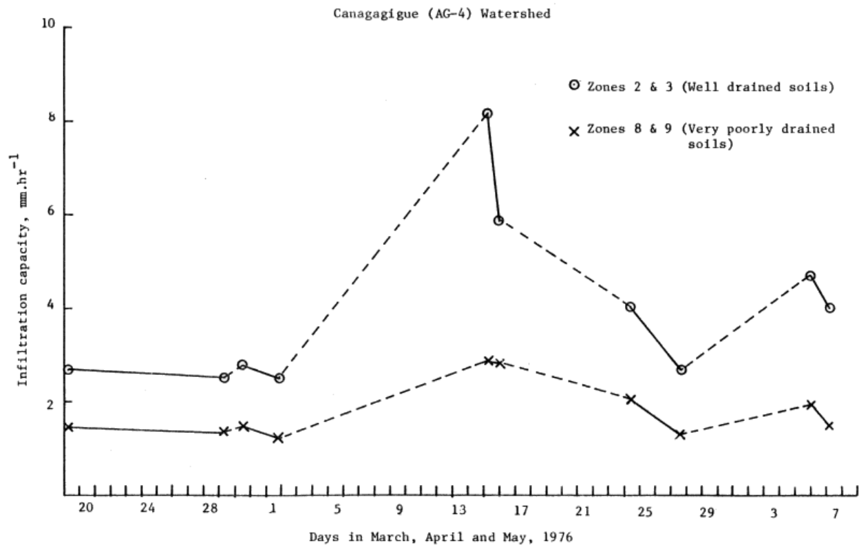
Fig. 37: Infiltration Capacity Rates During a Storm Sequence on Canagagigue (AG-4) Watershed for March - May, 1976.
