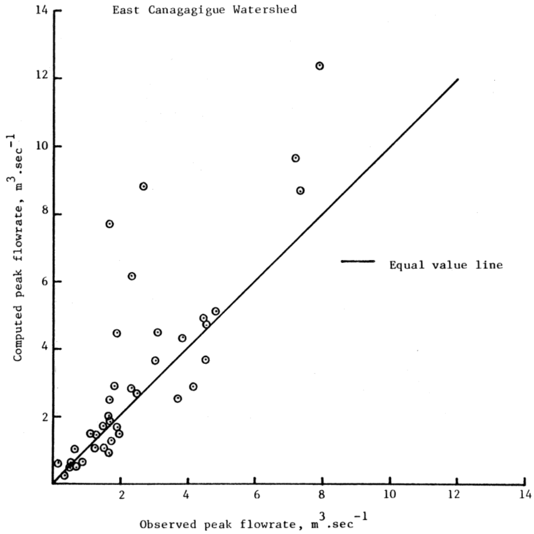
Fig. 21: Comparison of Observed and Computed Peak Flow-rates for Various Storms on East Canagagigue Watershed.
