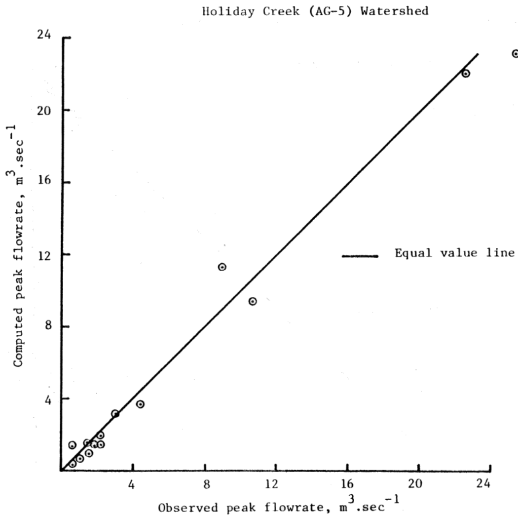
Fig. 22: Comparison of Observed and Computed Peak Flow-rates for Various Storms on holiday Creek (AG-5) Watershed.
