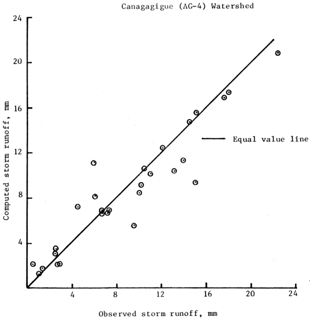
Fig. 23: Comparison of Observed and Computed Storm Runoff for Various Storms on Canagagigue (AG-4) Watershed.
