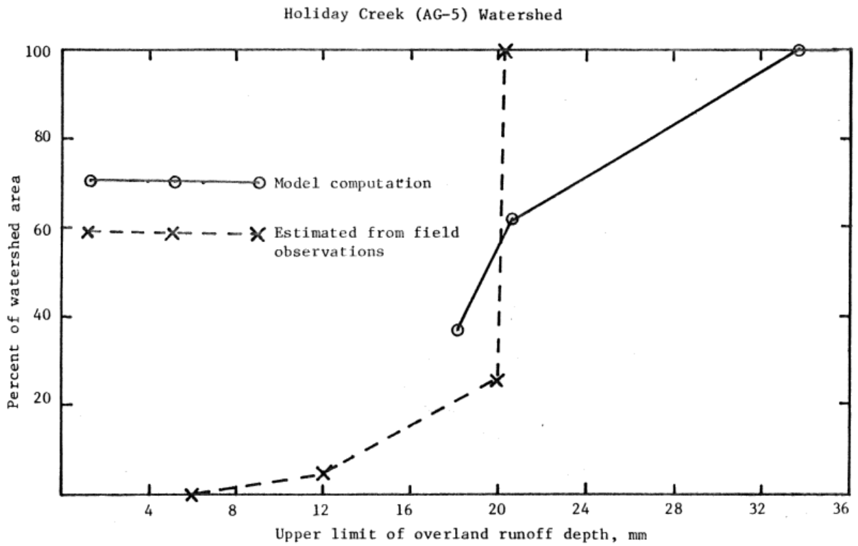
Figure 36: Comparison of estimated (field) and computed (model) overland-runoff depths produced during the August 13, 1976 storm on Holiday Creek (AG-5) watershed.
