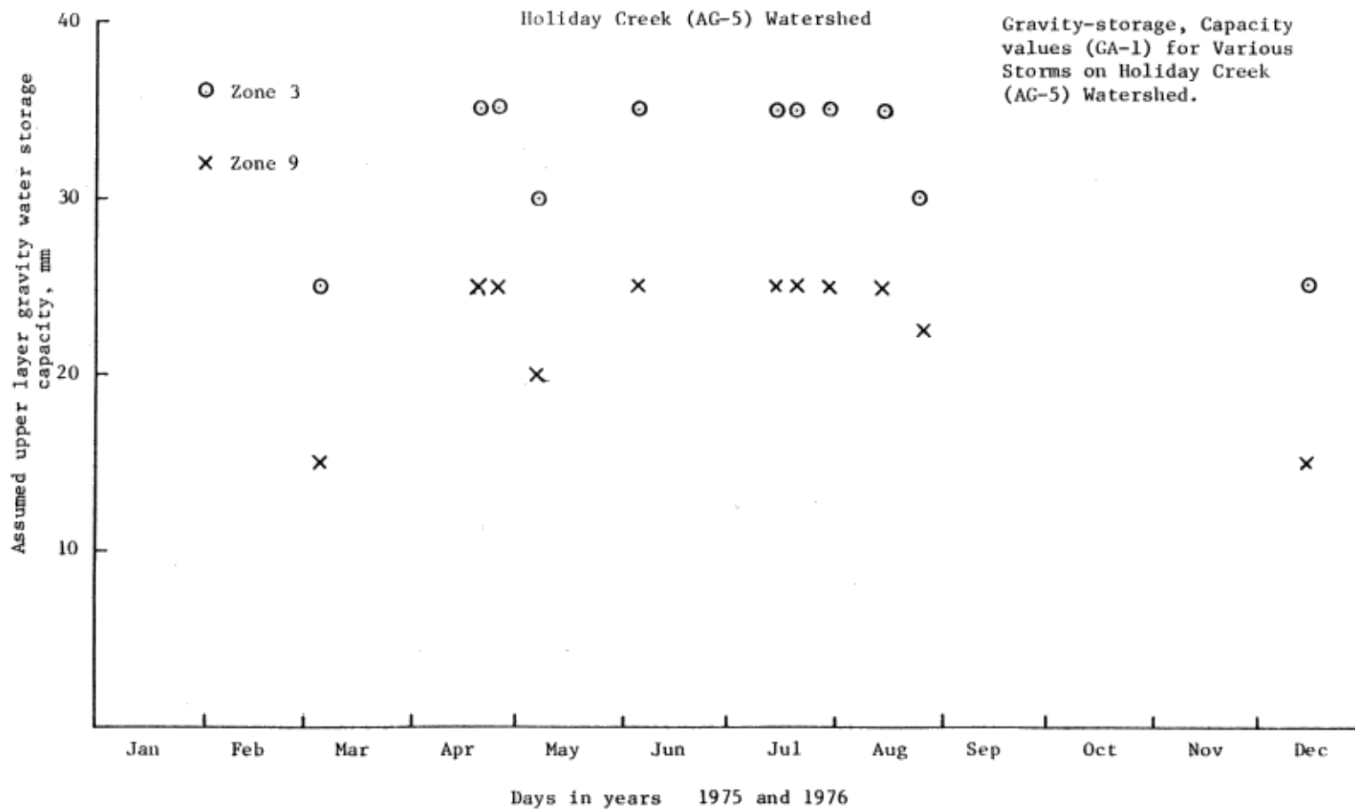
Fig. 15: Assumed Upper-layer, Gravity-storage, Capacity values (GA-1) for Various Storms on Holiday Creek (AG-5) Watershed.
