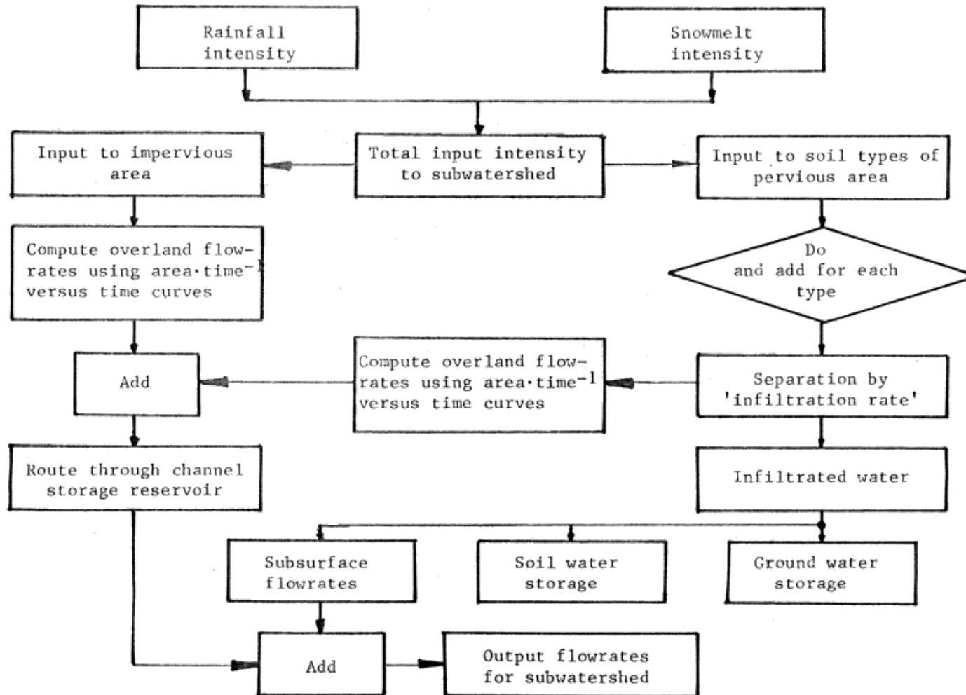
Fig. 12: Flowchart for Subwatershed Modeling.
