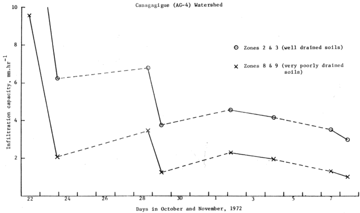
Fig. 38: Infiltration Capacity Rates During a Storm Sequence on Canagagigue (AG-4) Watershed for October - November, 1972.
