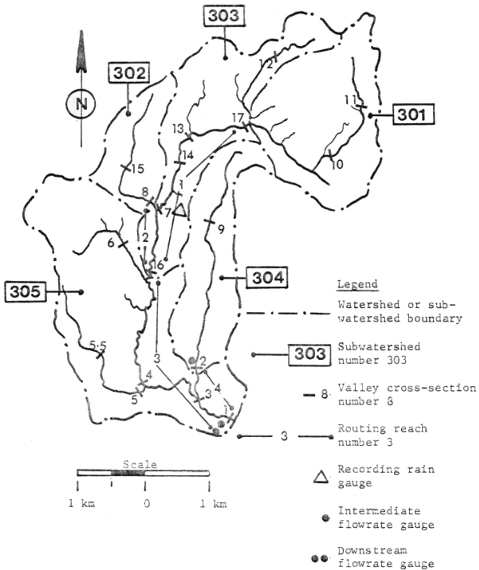
Fig. 1: Canagagigue (AG-4) Watershed near Floradale, Ontario.
