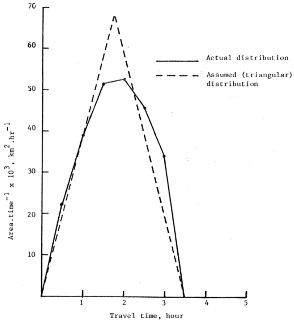
Figure 16: Actual and Approximated Area Time versus Time Curves for the Impervious Area of Subwatershed #306 of Holiday Creek (AG-5) Watershed when Watershed output Flowrate is 1.5 m 3 .sec -1 .
