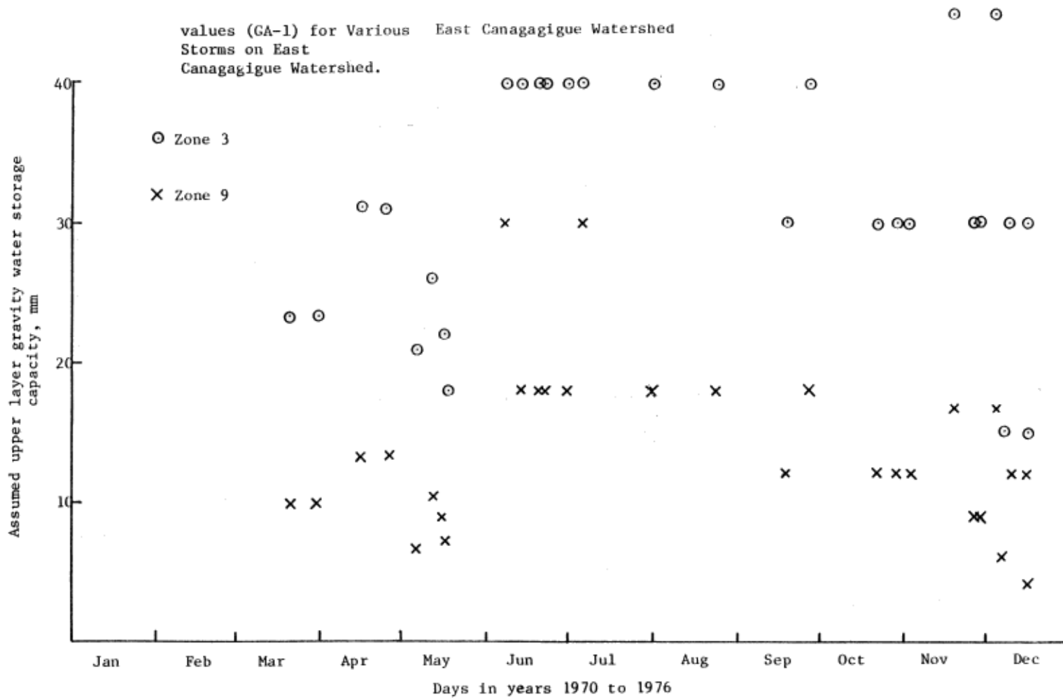
Fig. 14: Assumed Upper-layer, Gravity-storage, Capacity values (GA-1) for Various East Canagagigue Watershed Storms on East Canagagigue Watershed.
