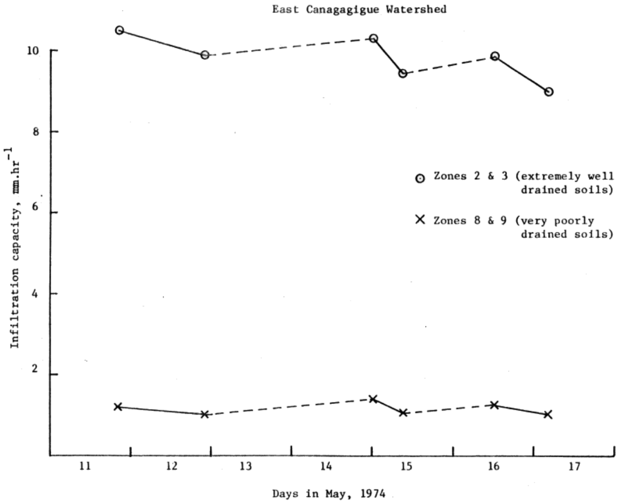
Fig. 39: Infiltration Capacity Rates During a Storm Sequence on East Canagagigue Watershed for May, 1974.
