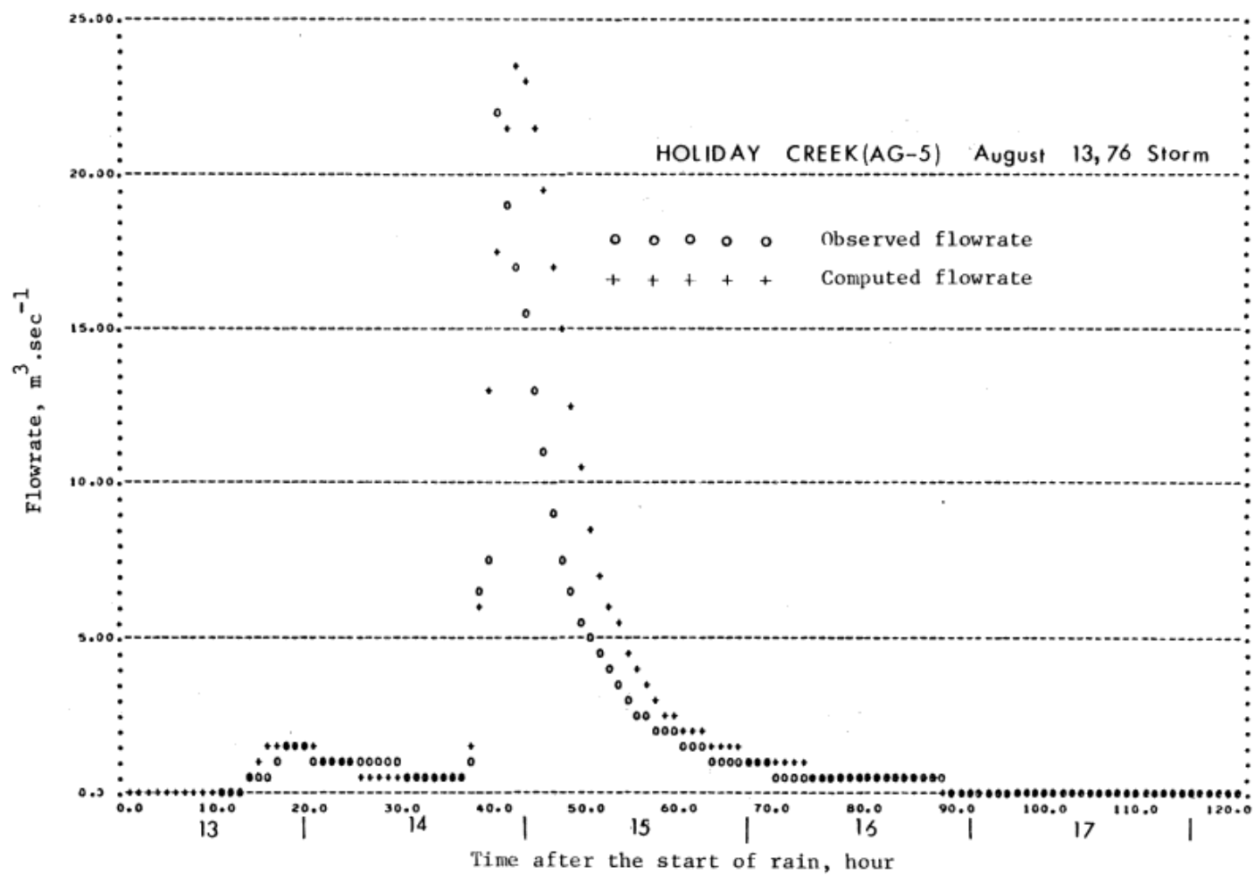
Fig. 19: Comparison of Observed and Simulated Flowrates due to August 13, 1976 Storm on Holiday Creek (AG-5) Watershed.
