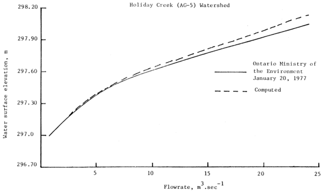
Fig. 6: Comparison of Recorded and Computed Rating Curves at the Downstream Gauging Station (at Cross-section 1) of Holiday Creek (AG-5) Watershed.
