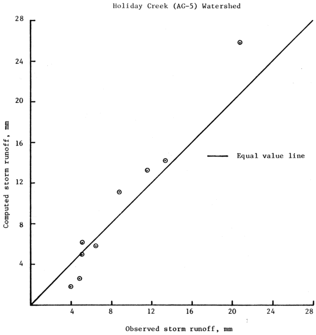
Fig. 25: Comparison of Observed and Computed Storm Runoff for Various Storms on Holiday Creek (AG-5) Watershed.
