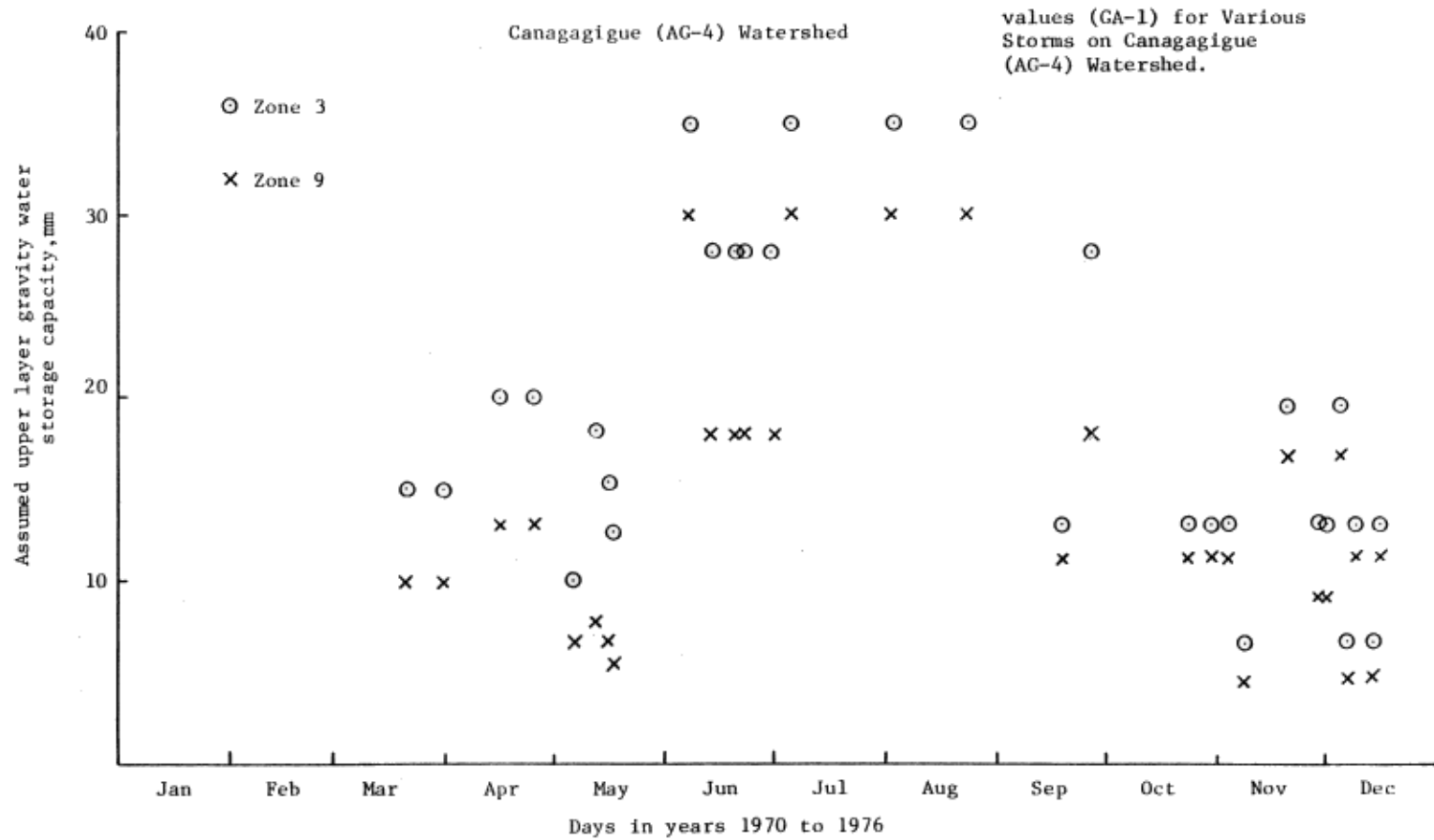
Fig. 13: Assumed Upper-layer, Gravity-storage, Capacity values (GA-1) for Various Storms on Canagagigue (AG-4) Watershed.
