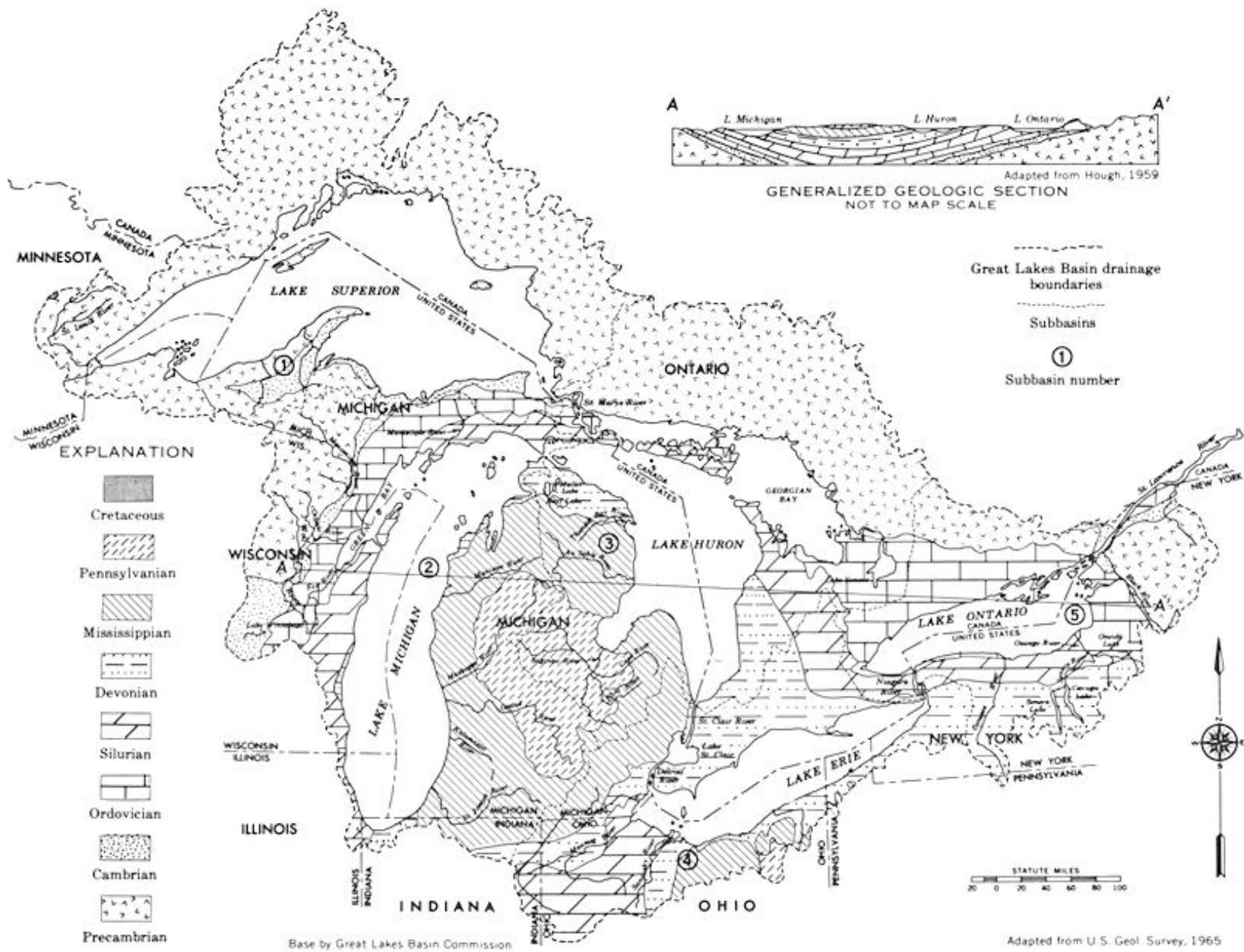
FIGURE 2: Bedrock Geology of the Great Lakes Basin 2
