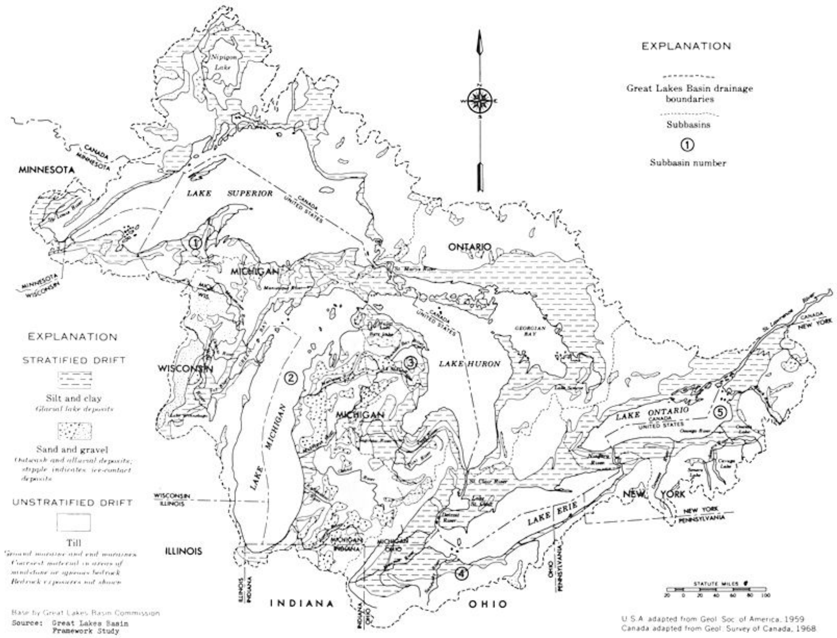
FIGURE 3: Glacial Geology of the Great Lakes Basin 2
