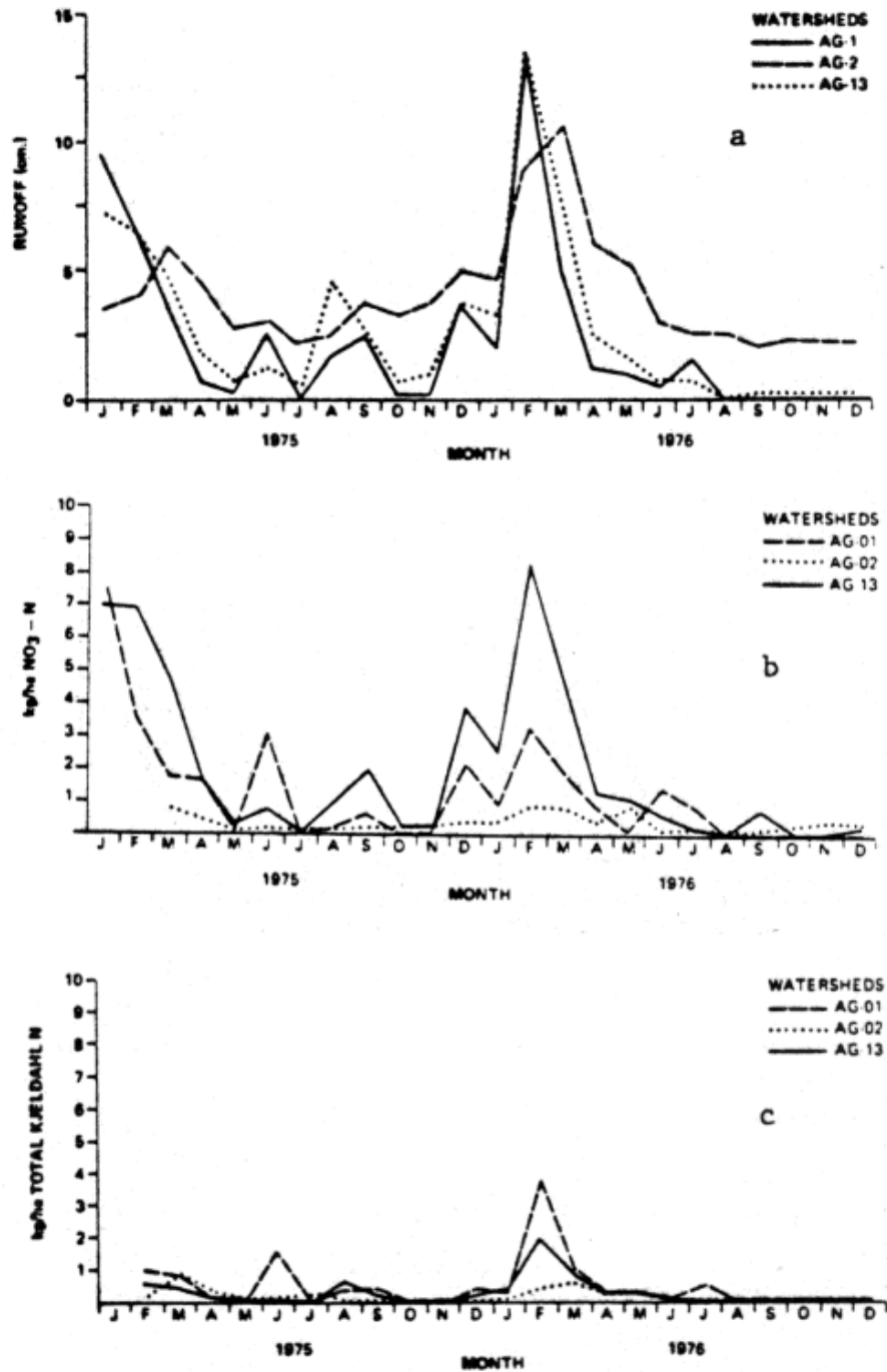
Fig. 5-4 Monthly runoff and Naquadat NO 3 -N and TKN loadings for agricultural watersheds AG-01, AG-02 and AG-13, 1975-1976.
