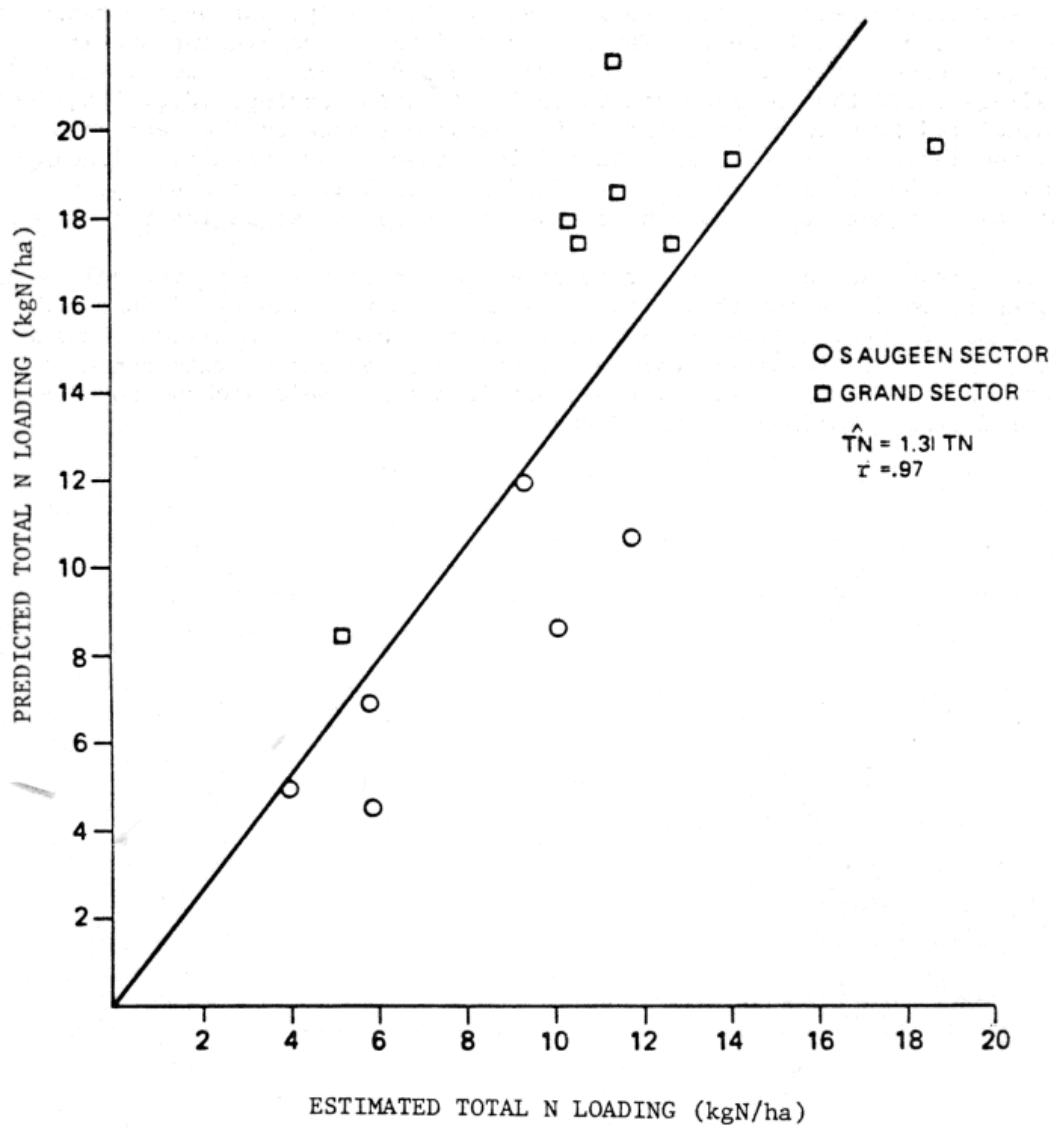
Fig. 7-5. Comparison of predicted 1975-1976 unit Total-N loadings with those estimated using Beale ratio estimator technique.
