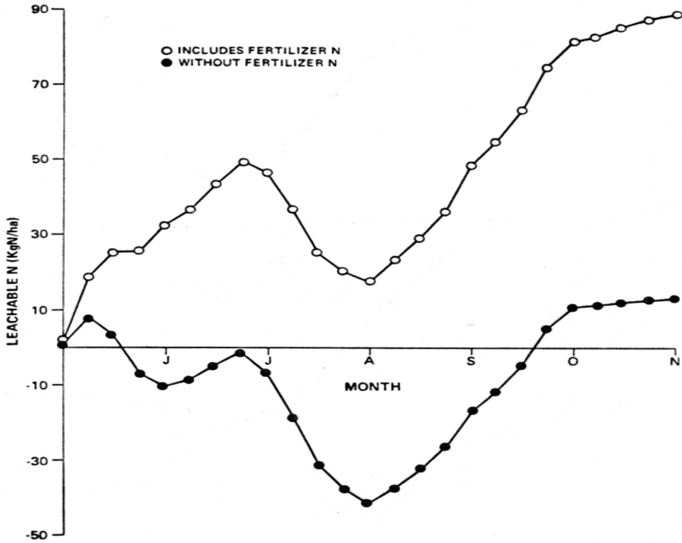
Fig. 7-2. Soil N potentially leachable from AG-05.
