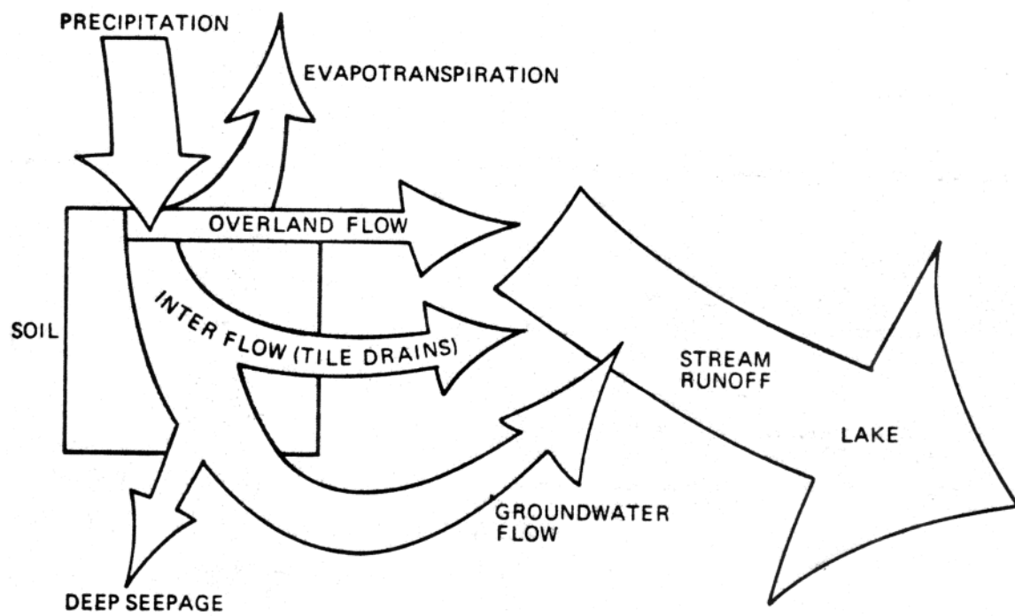
Fig. 2-1. Schematic of hydrologic cycle illustrating major watershed runoff routes.
