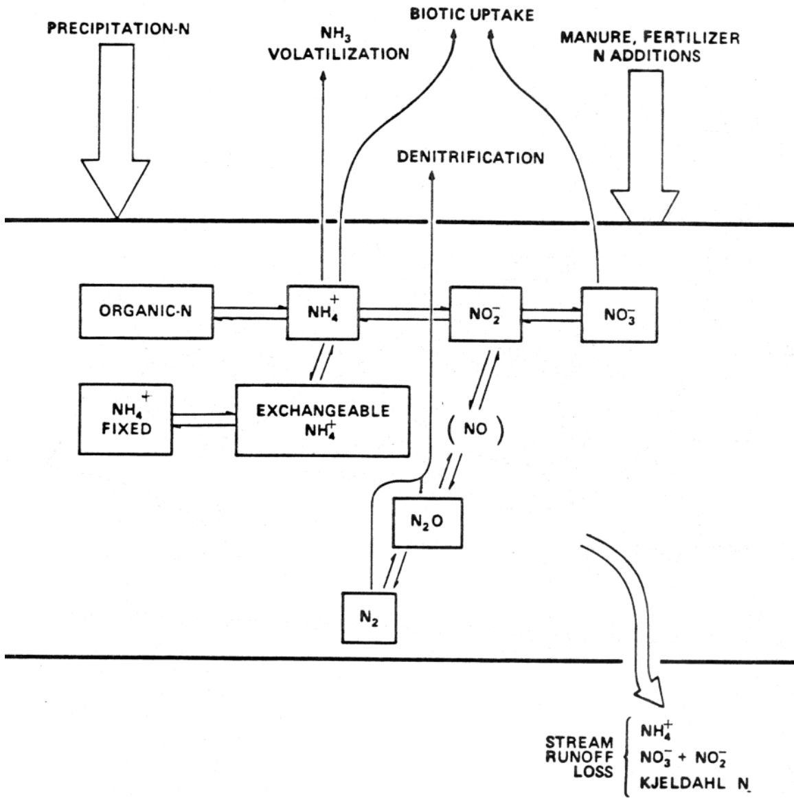
Fig. 2-2. Major chemical pathways involved in N cycle.
