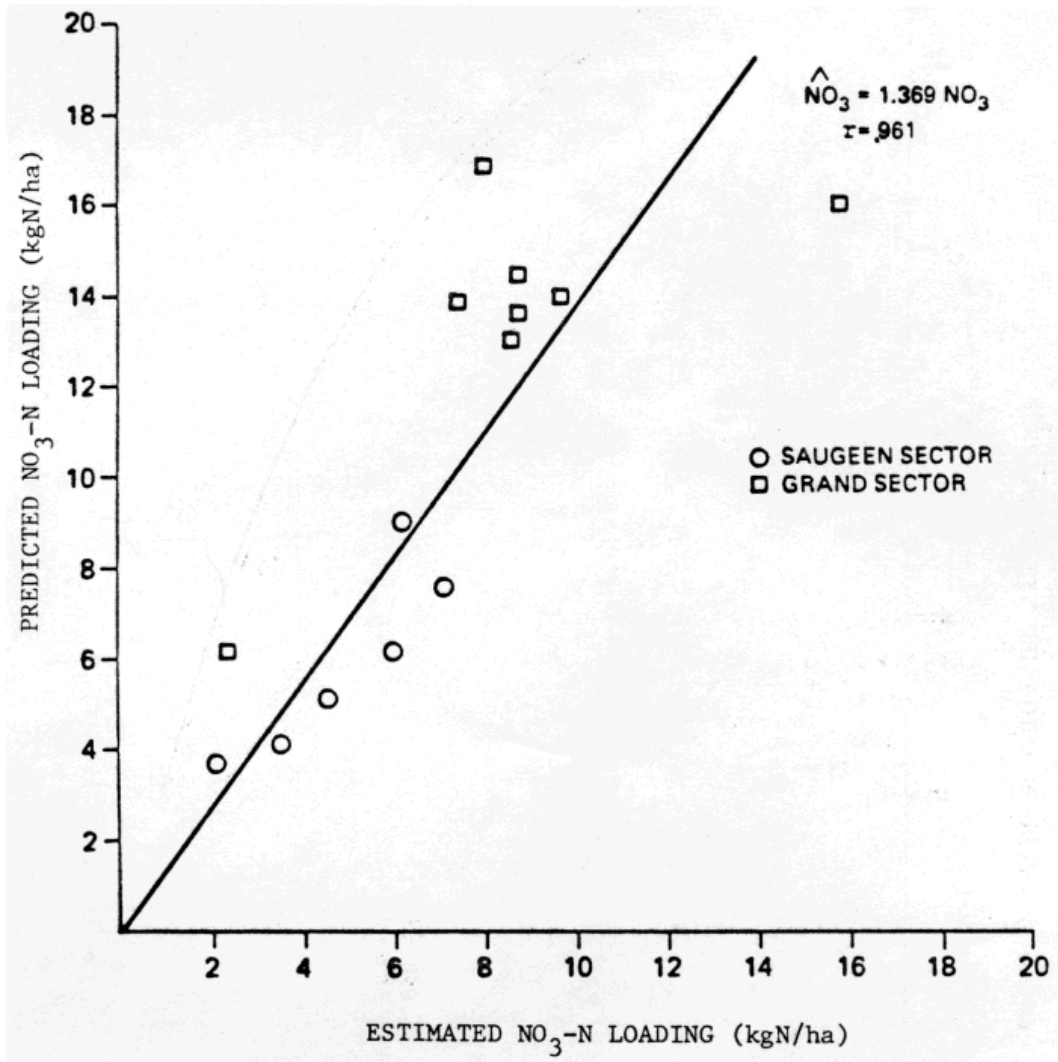
Fig. 7-6. Comparison of predicted 1975-1976 unit NO 3 -N loadings with those estimated using the Beale ratio estimator technique.
