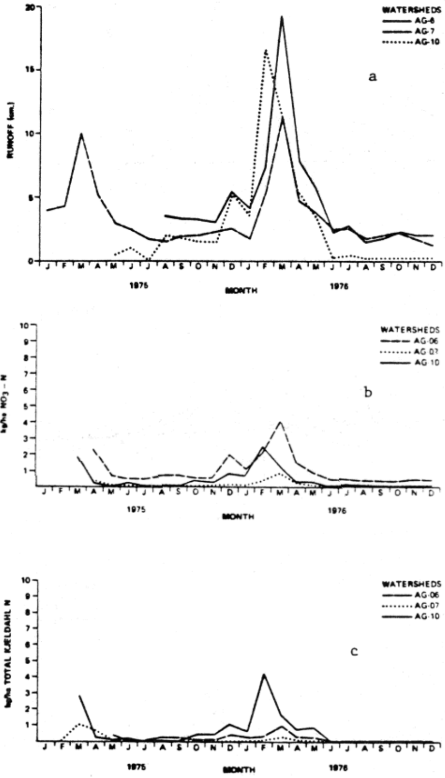
Fig. 5-5 Monthly runoff and Naquadat \text{NO}_3\text{-N} and TKN loadings for agricultural watersheds AG-06, AG-07 and AG-10.
