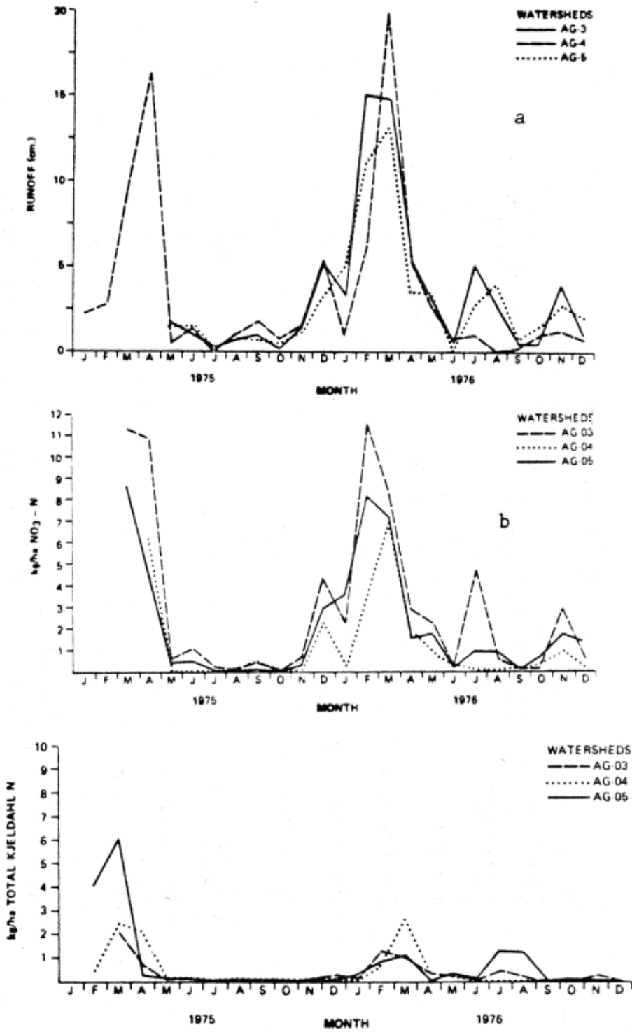
Fig. 5-3 Monthly runoff and Naquadat NO 3 -N and TKN loadings for agricultural watersheds AG-03, AG-04 and AG-05, 1975-1976.
