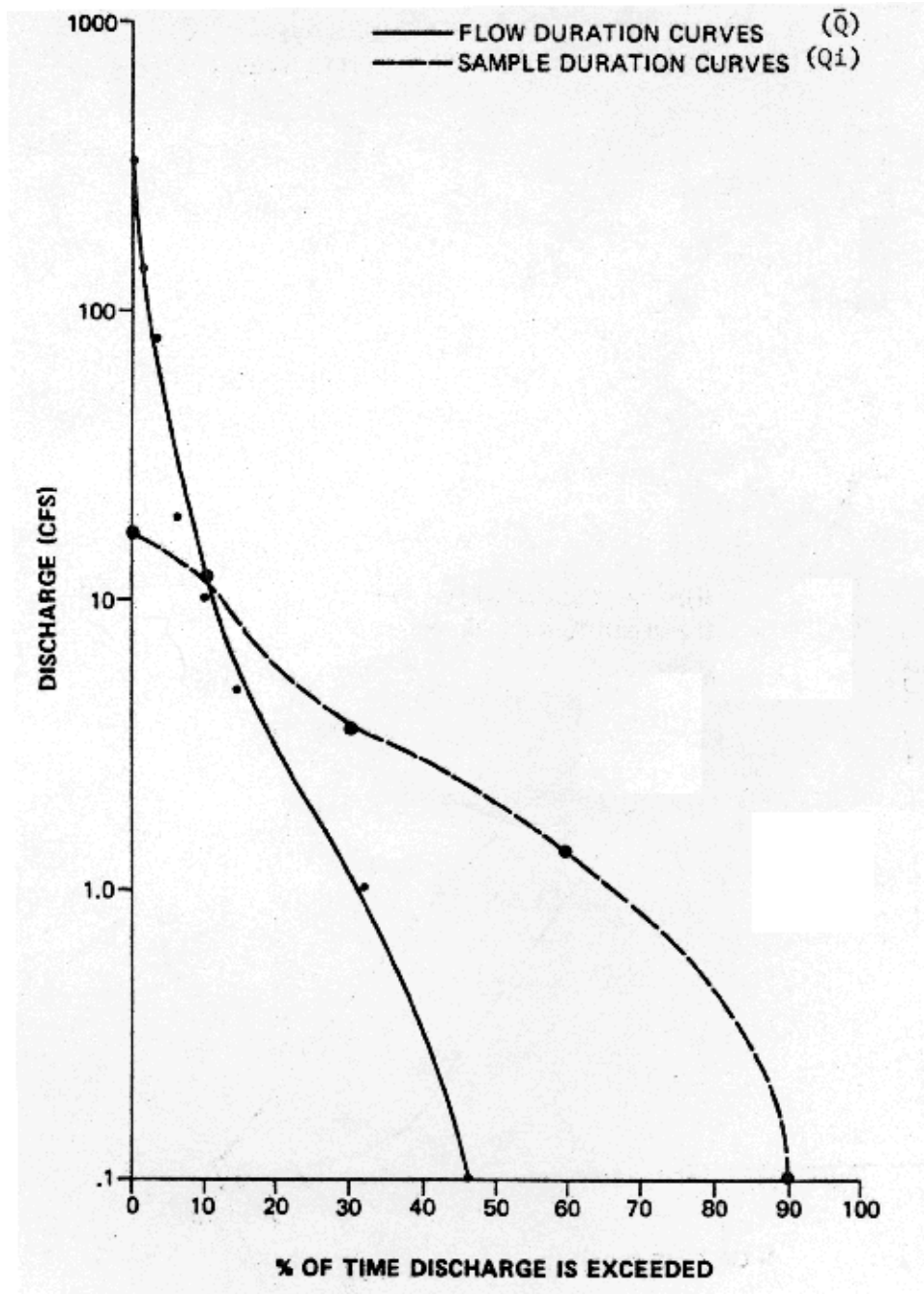
Fig. A-3-9 Flow duration curve based on mean daily discharge ( \bar{Q} ) and sample duration curve based on instantaneous discharge ( Q_i ) for Watershed AG-11.
