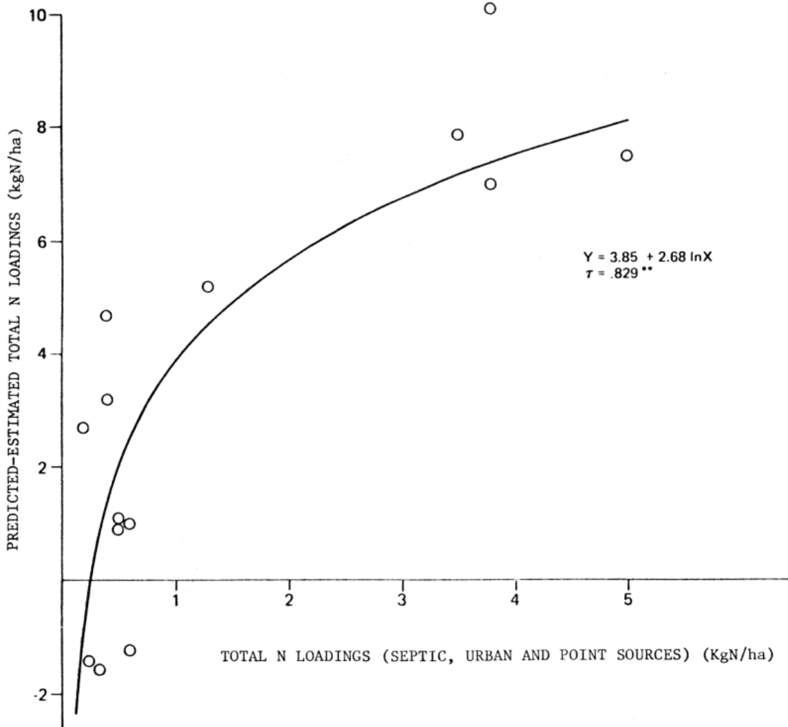
Fig. 7-7. Relationship between the residual of predicted and estimated stream loadings of N from agriculture and nonagricultural total N inputs.
