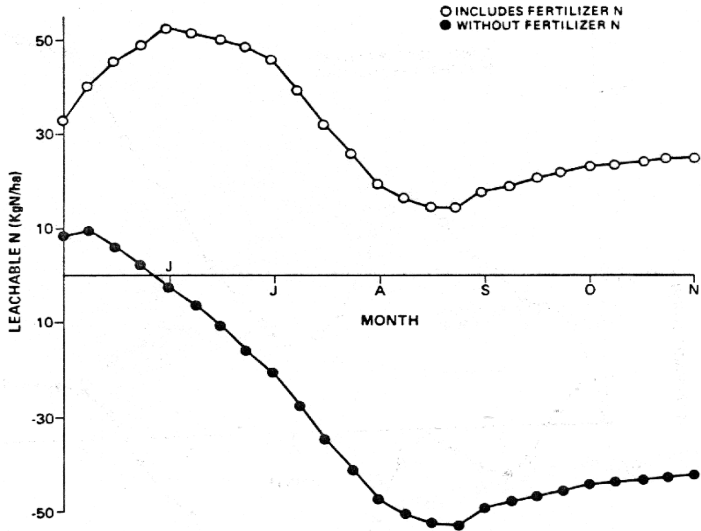
Fig. 7-3. Soil N potentially leachable from AG-13 in 1975.
