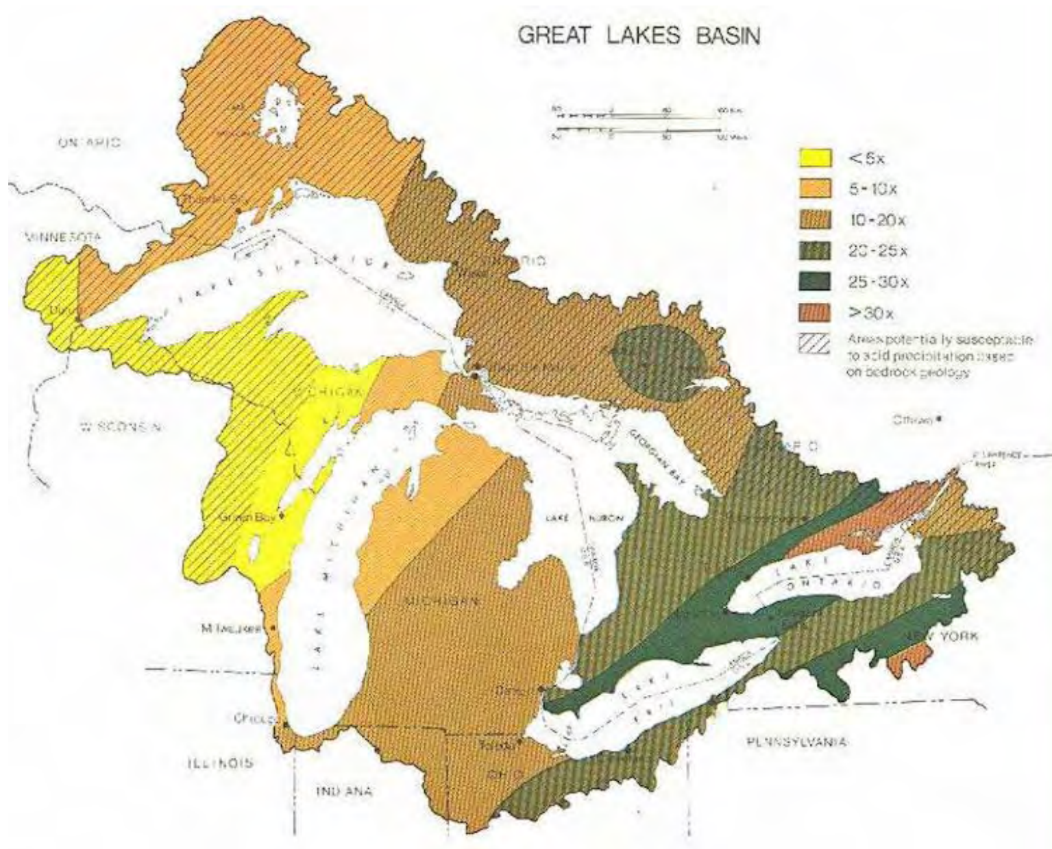
Fig. 2. Increased Acidity In Bulk Precipitation Over Natural Concentration (pH 5.7)
