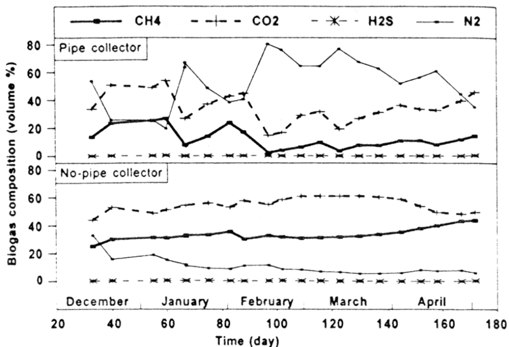
Figure 6. Average biogas composition in pipe and no-pipe gas collectors during winter. Gas concentration peaks in the pipe-system biogas resulted from introduction of air into the floating covers when they were removed from the pipes for monthly collection of slurry samples from inside the pipes.
