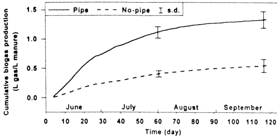
Figure 5. Average cumulative biogas production under pipe and no-pipe gas collectors in the manure tank during summer.
