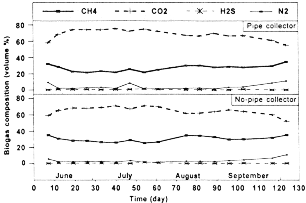
Figure 7. Average biogas composition in pipe and no-pipe gas collectors during summer.
