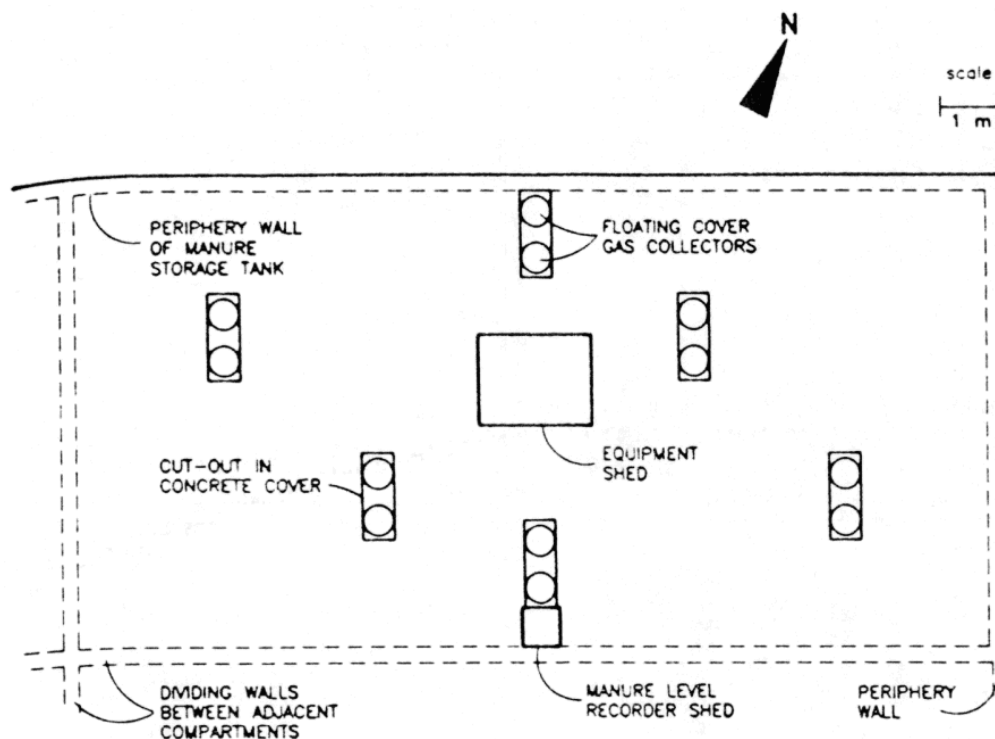
Figure 1. Layout of the six replicate sites for floating-cover biogas collectors, data-logging equipment shed, and manure level recorder shed at the 7.2 x 14.7 x 2.8 m deep below-grade manure slurry storage tank. This tank formed one compartment of a four-compartment concrete tank.
