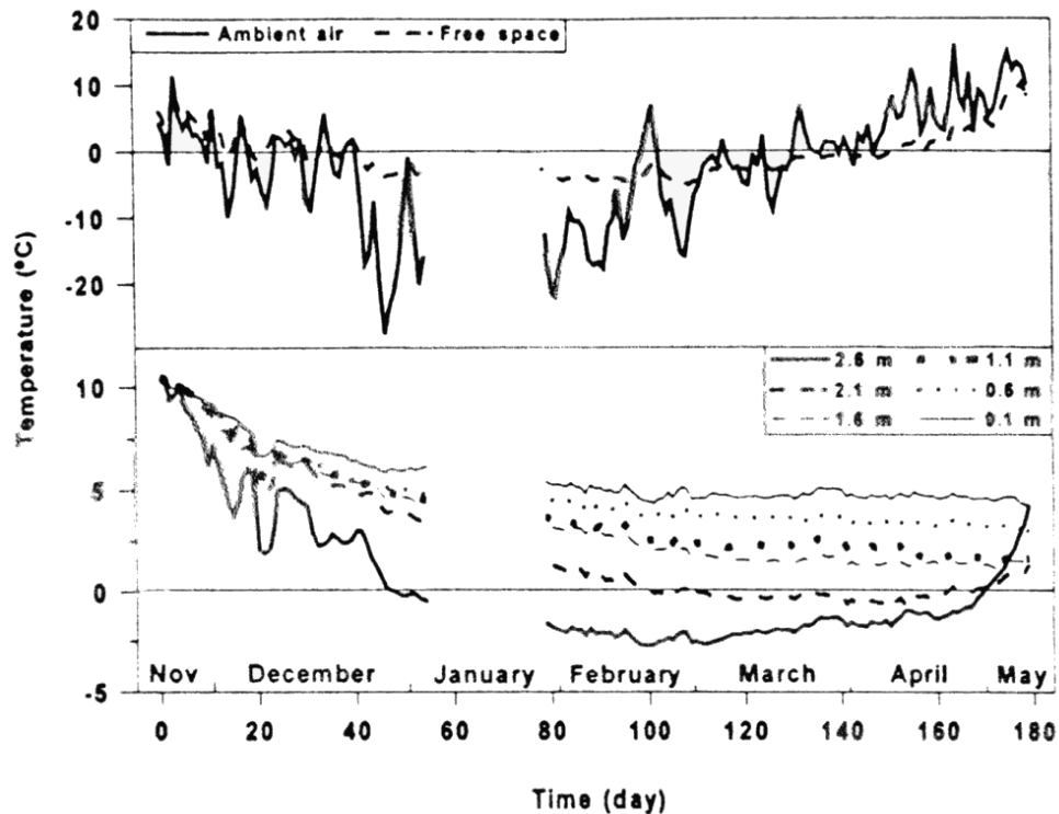
Figure 3. Ambient temperature, and average slurry and free-space temperature during the winter. Slurry temperature is shown at various distances from the bottom. Temperature recording was interrupted in January to install a new datalogging system.
