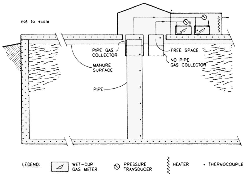
Figure 2. Section through manure tank showing the pipe and no-pipe biogas collection systems.
