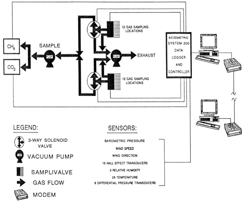
Figure 2. Gas sampling system and data acquisition and control system
