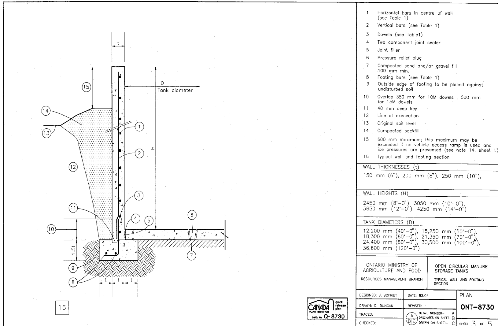
Figure 3 Tank wall detail from Plan ONT-8730 showing wall, footing, floor (1992)
