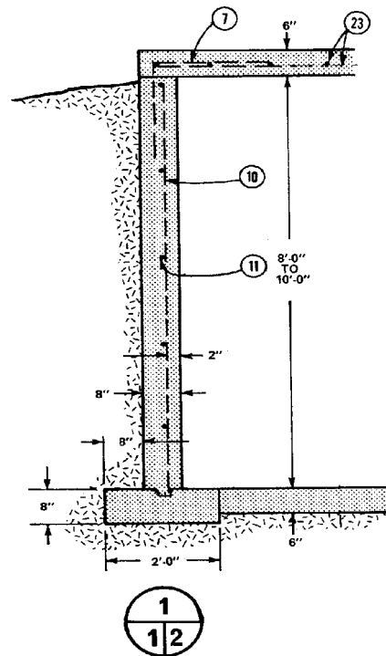
Figure 2 Detail from Canada Plan Service Plan 8712 showing cross-section of in-ground concrete tank with typical wall, footing, floor, and roof details
