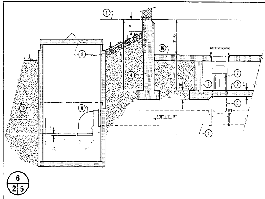
Figure 4 Detail from Canada Plan Service plan 3303 showing Saddle-T pipe connection (item 6) and horizontal drain pipe (item 5) in flush gutter system
